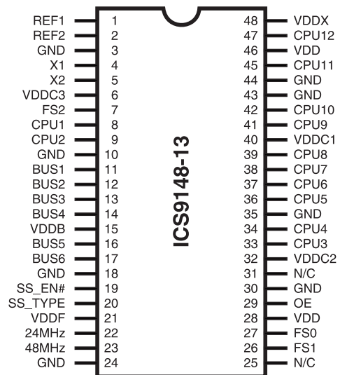
48-Pin SSOP
