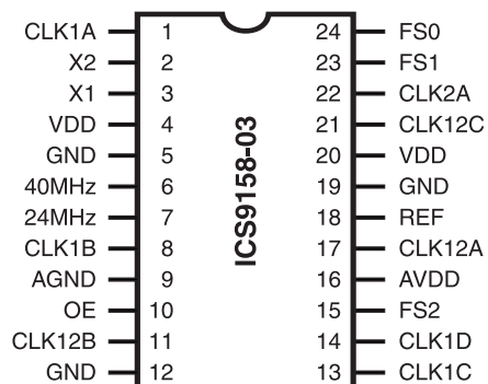
24-Pin SOIC
