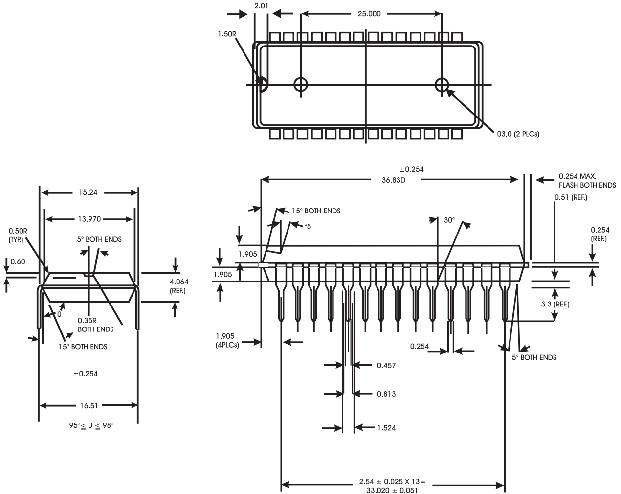
28-Pin DIP Package
