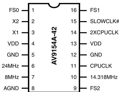
16-Pin PDIP or SOIC AV9154A-42
