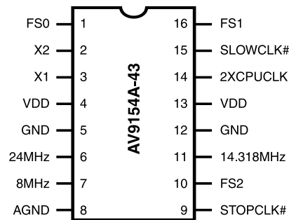
16-Pin PDIP or SOIC AV9154A-43
