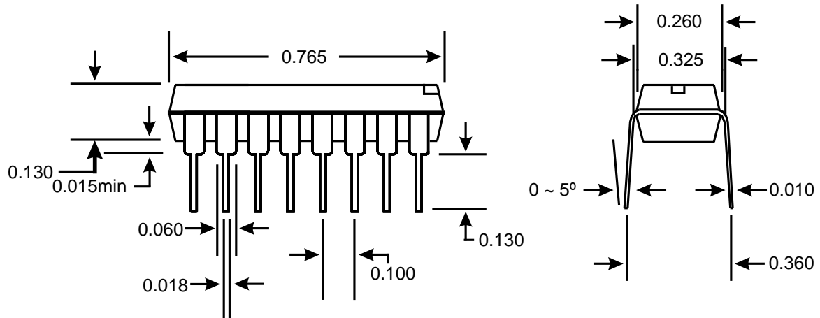
16-Pin PDIP Package
