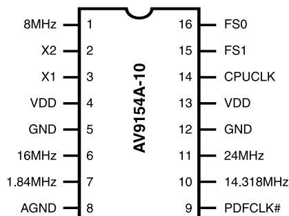
16-Pin PDIP or SOIC 9154-10
