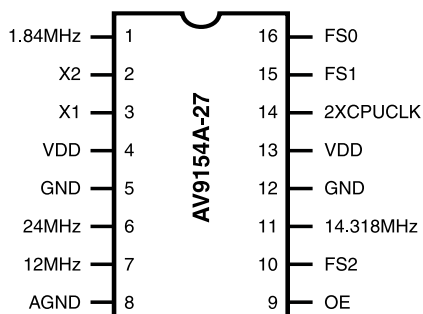
16-Pin PDIP or SOIC AV9154A-27
