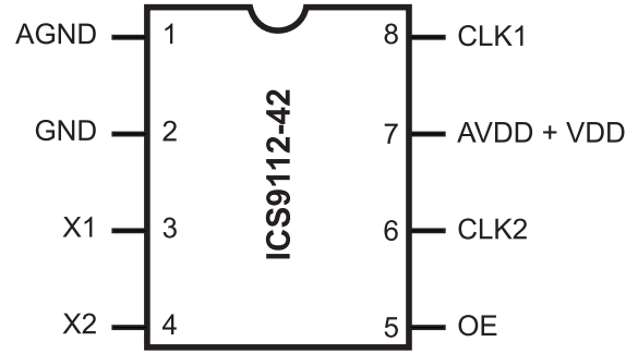
8-Pin SOIC
