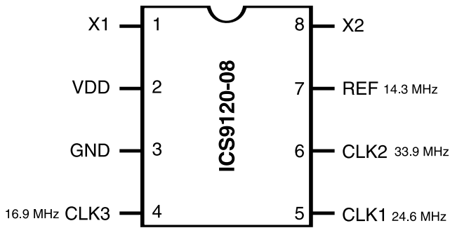
8-Pin SOIC
