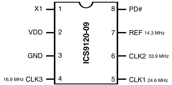
8-Pin SOIC
