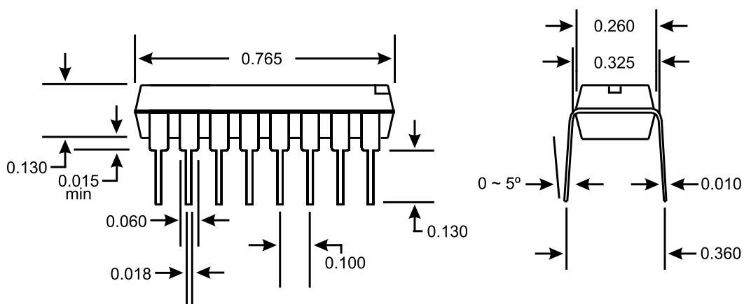
16-Pin DIP Package
