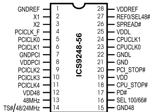
28 pin SSOP and TSSOP
