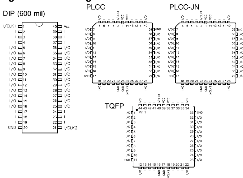
Figure 1: Pin Configuration
