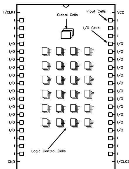
Figure 2. Block Diagram
