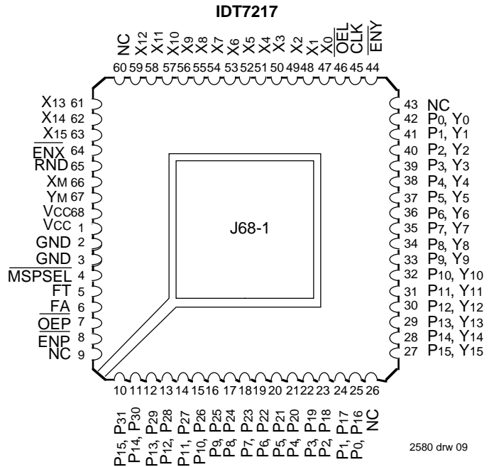
PLCC TOP VIEW
