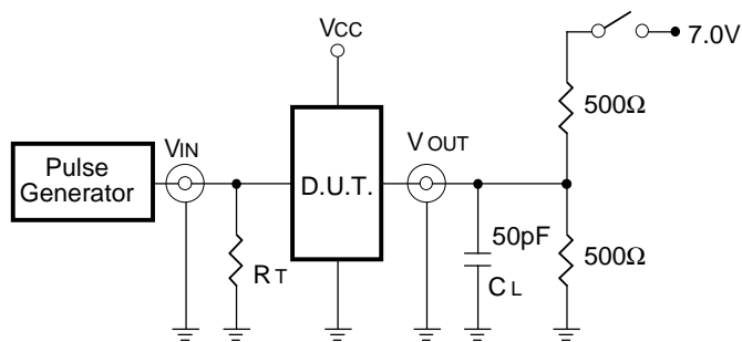
Figure 12. AC Test Load Circuit
