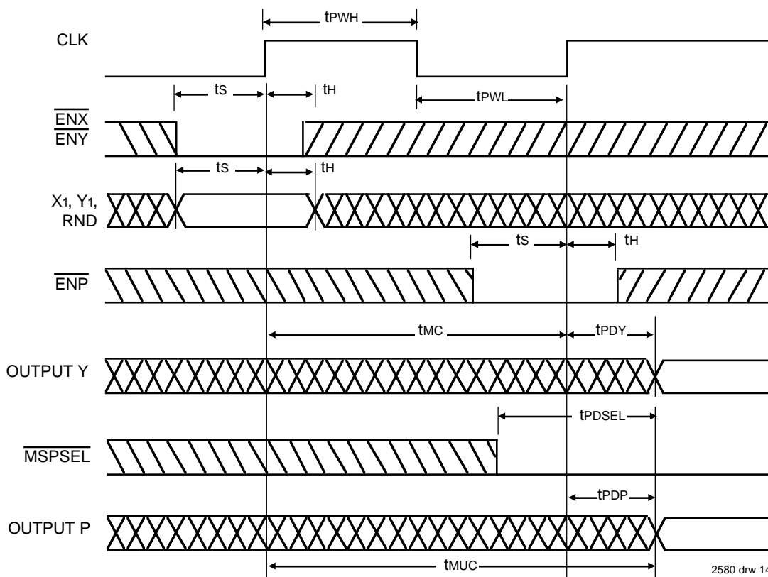
Figure 5. IDT7217 Timing Diagram
