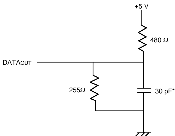
Figure 1. Output Load
