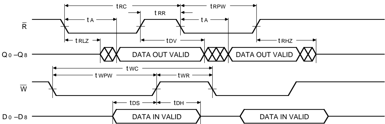
Figure 3. Asynchronous Write and Read Operation
