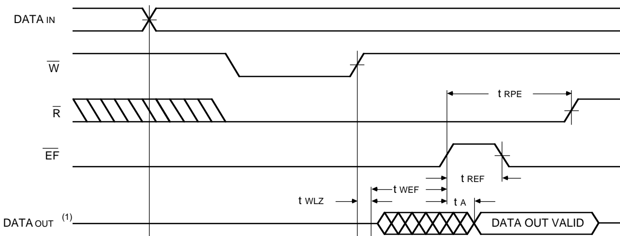
Figure 18. Read Data Flow-Through Mode
