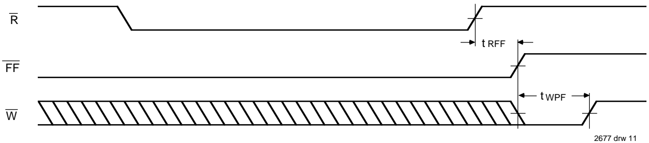
Figure 8. Full Flag Timing
