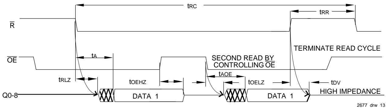
Figure 10. Output Enable and Read Operation Timings
