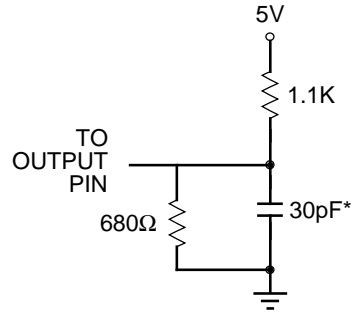
or equivalent circuit Figure 1. Output Load
