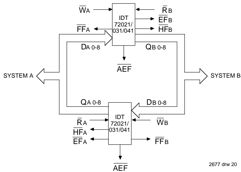
Figure 17. Bidirectional FIFO Mode
