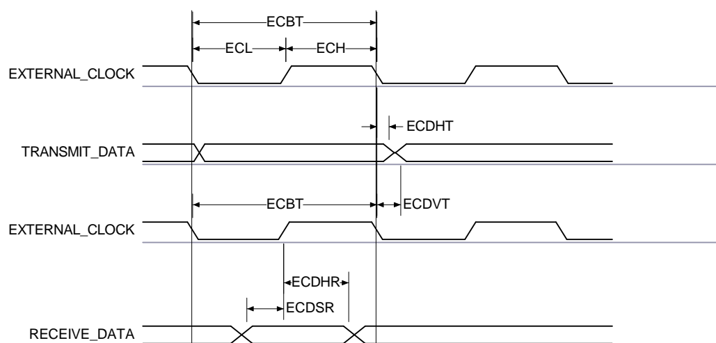
Figure 13: GSC Timings (External Clock)
