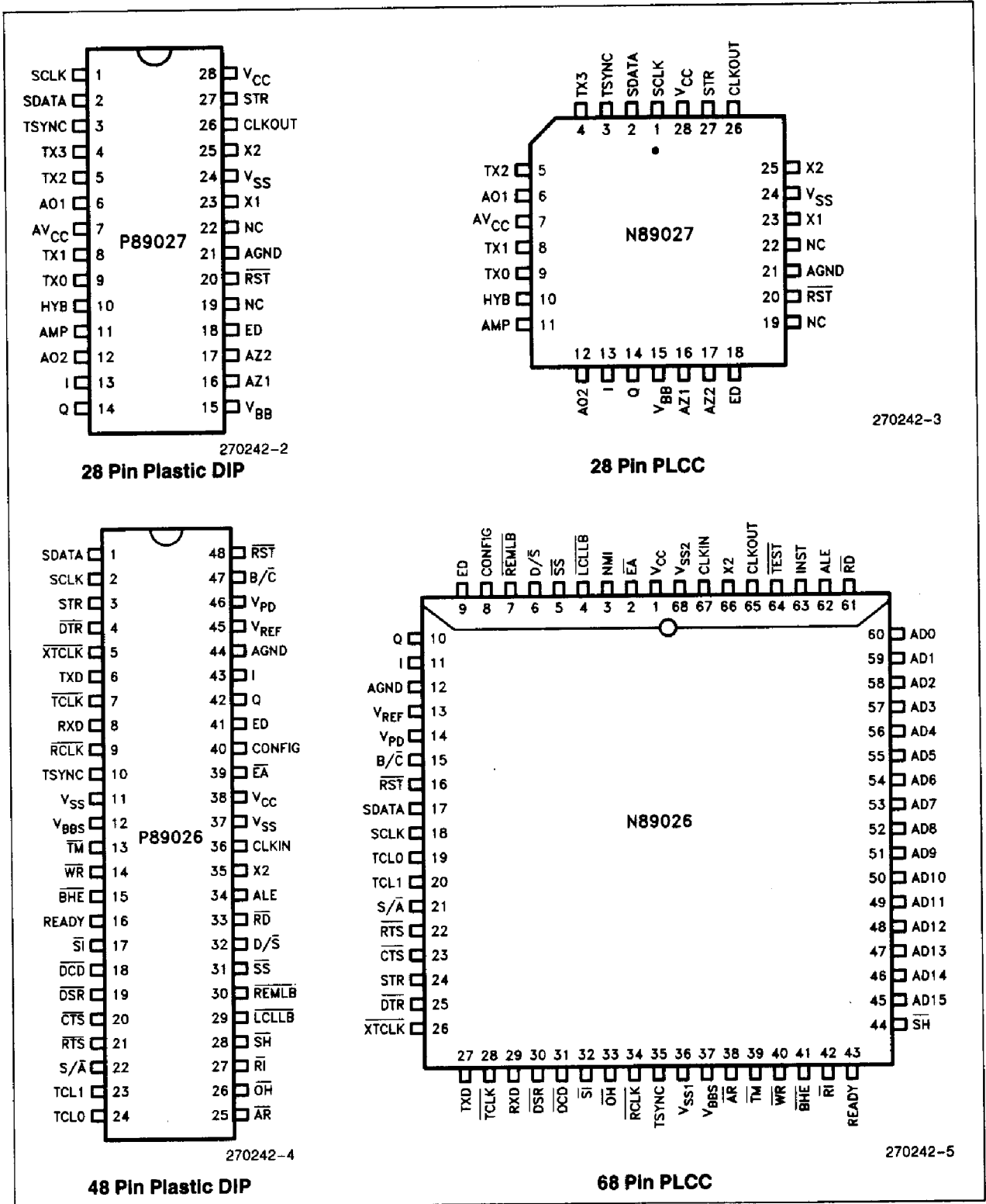
Figure 2. Device Packages
