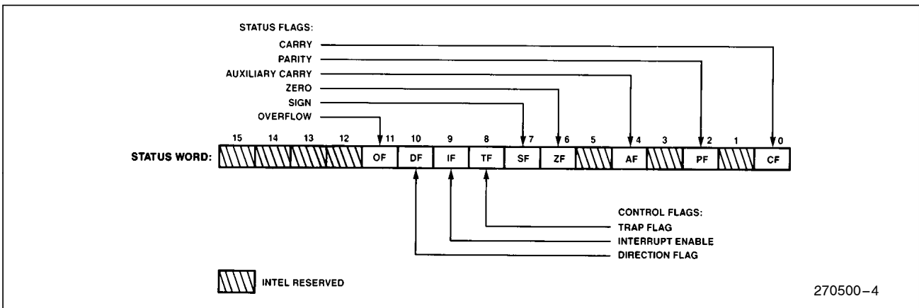
Figure 3b. Status Word Format
