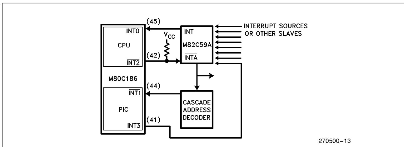
Figure 33. Slave Mode Interrupt Controller Connections
