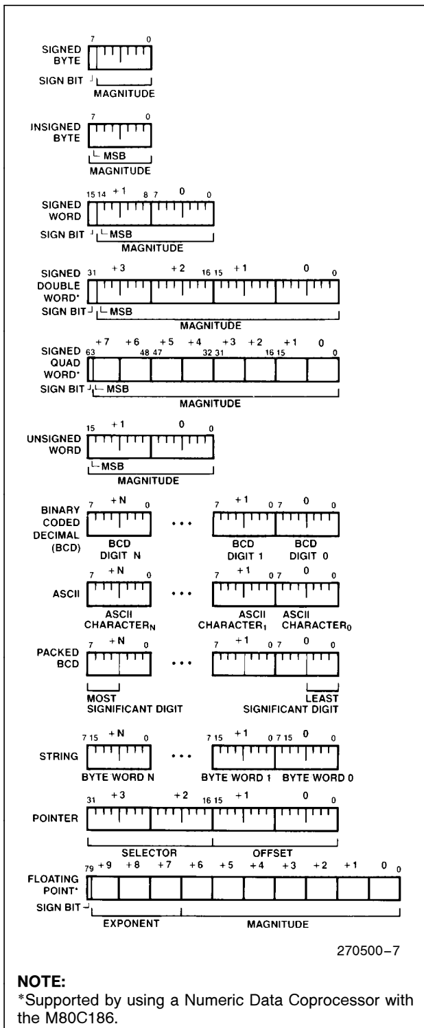
Figure 7. M80C186 Supported Data Types
