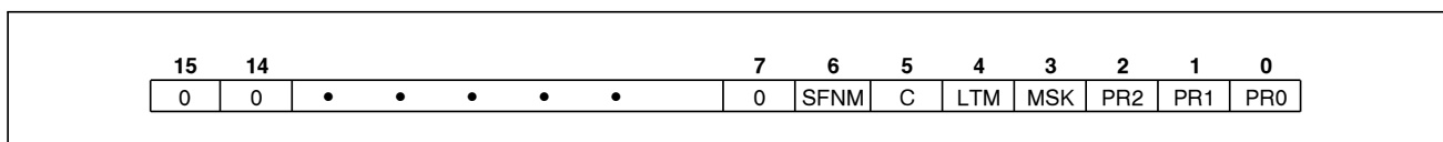
Figure 29. INT0/INT1 Control Register Formats
