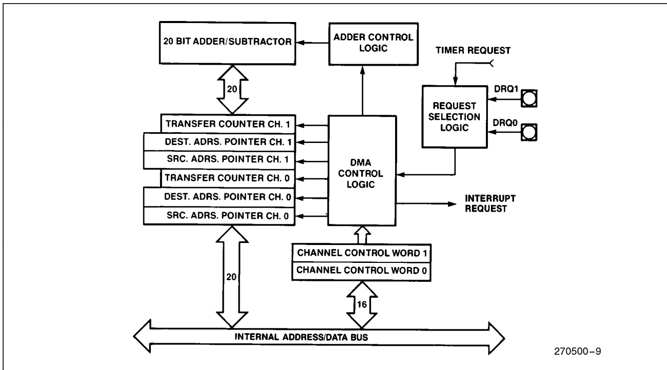
Figure 16. DMA Unit Block Diagram
