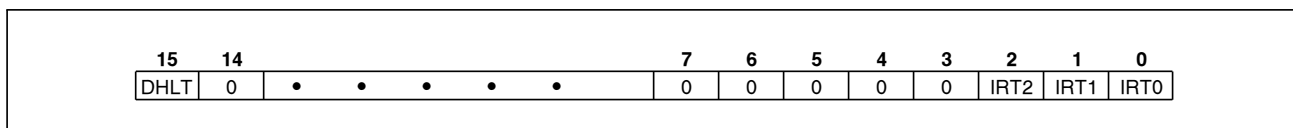
Figure 27. Interrupt Status Register Format (Master Mode)
