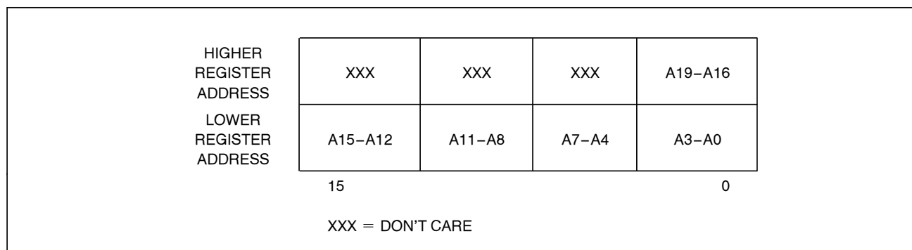
Figure 18. DMA Memory Pointer Register Format
