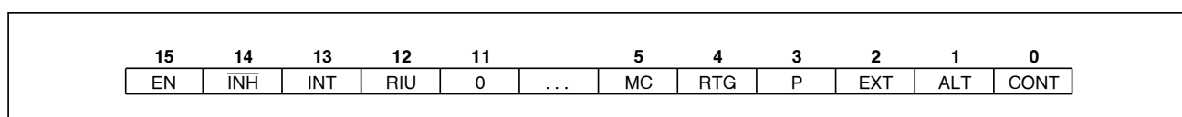
Figure 20. Timer Mode/Control Register
