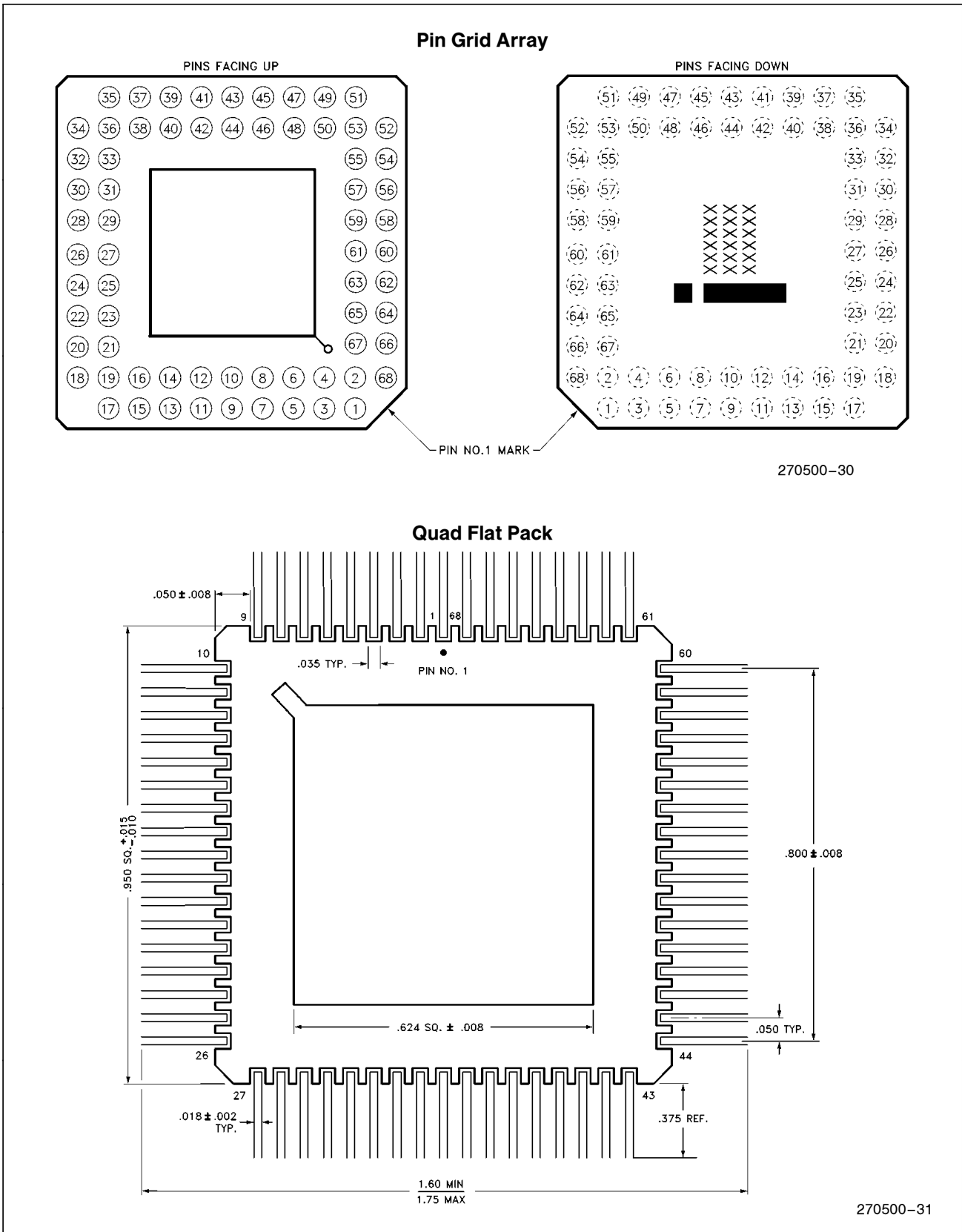
Figure 2. M80C186 Pinout Diagram
