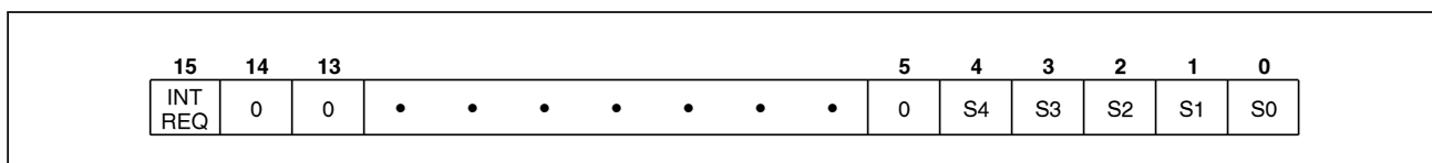
Figure 32. Poll and Poll Status Register Format
