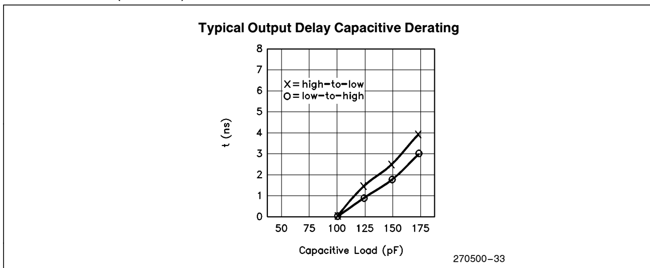
Figure 45. Capacitive Derating Curve
