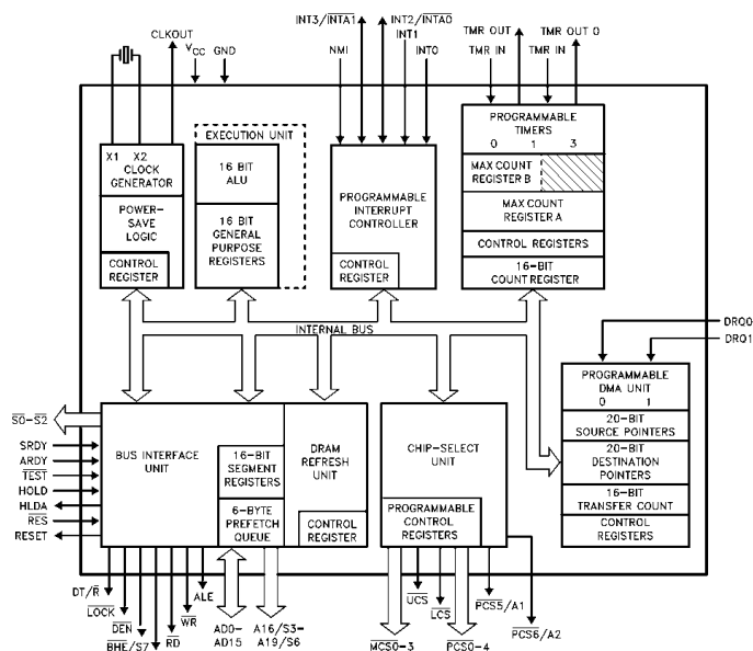
Figure 1. M80C186 Block Diagram
