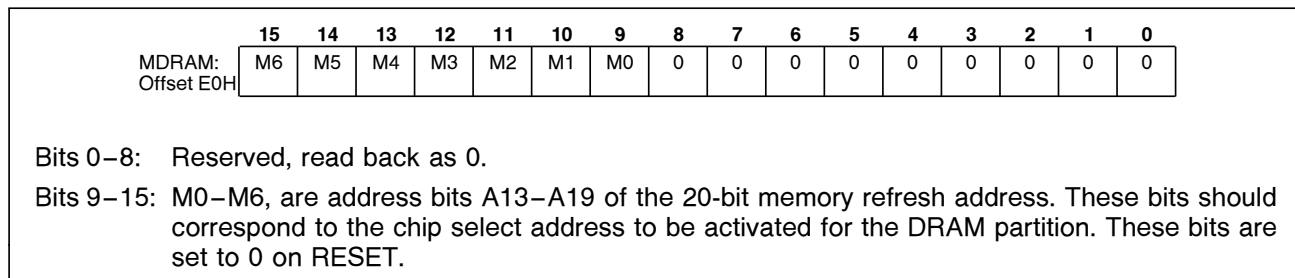
Figure 40. Memory Partition Register
