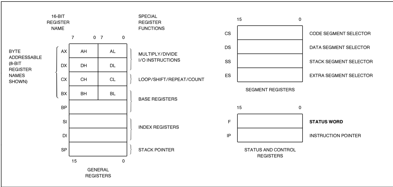
Figure 3a. M80C186 Register Set
