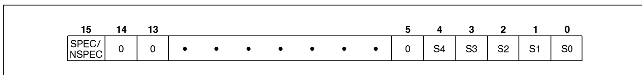
Figure 31. EOI Register Format
