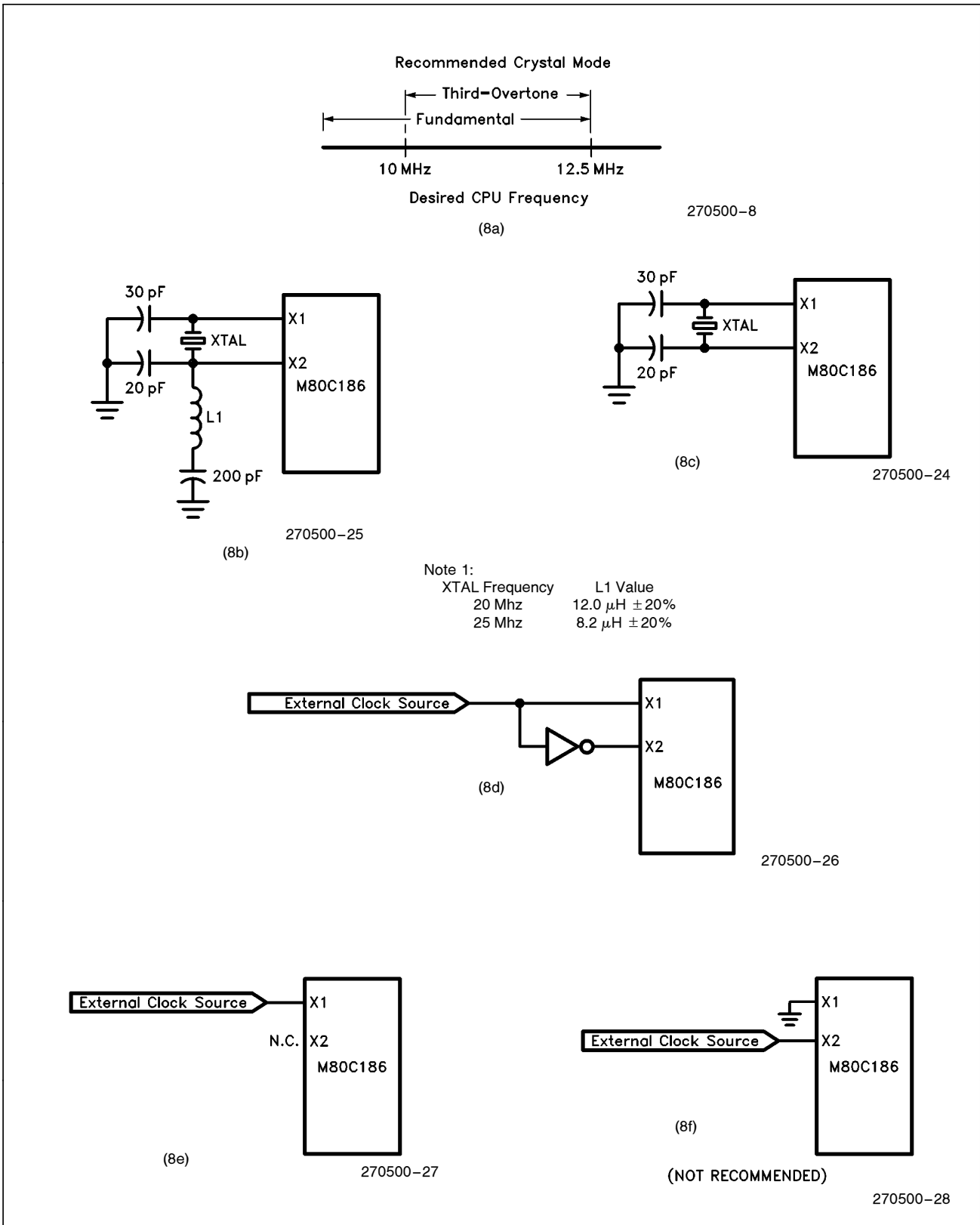
Figure 8. M80C186 Oscillator Configurations
