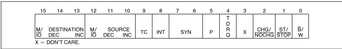
Figure 17. DMA Control Register
