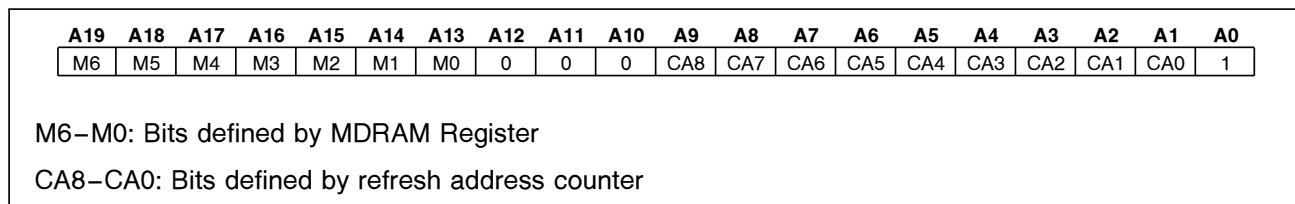
Figure 41. Addresses Generated by RCU
