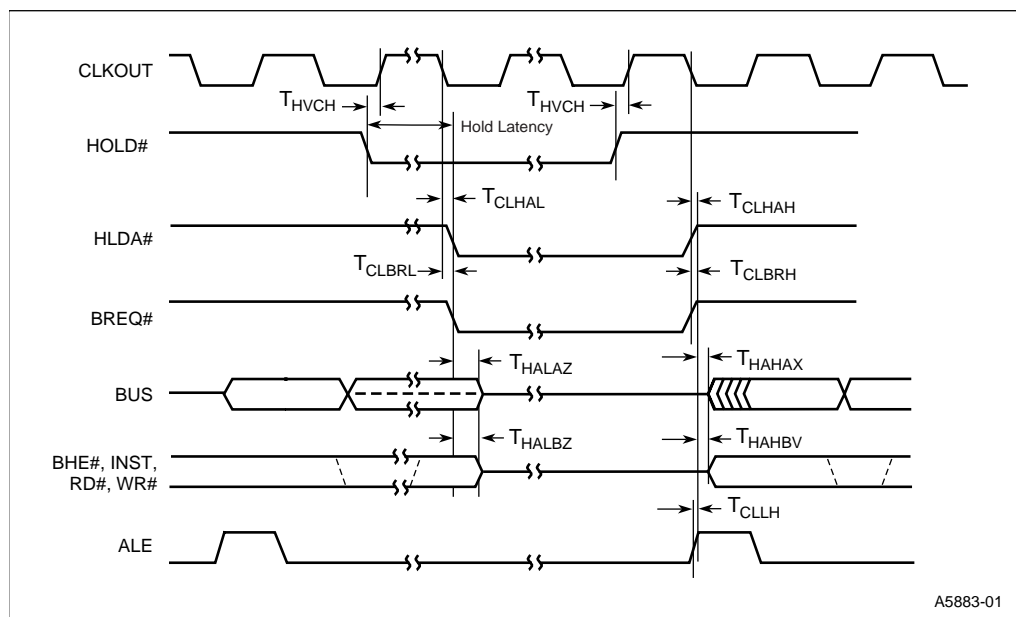
Figure 17. HOLD Timings
