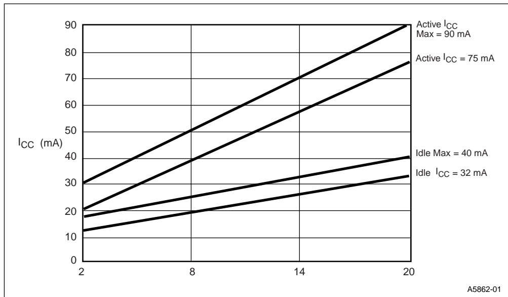
Figure 8. 87C196CA I CC vs. Frequency
