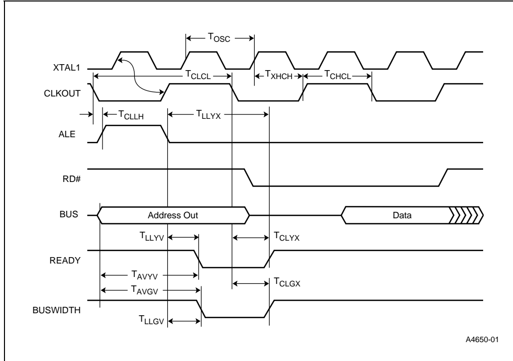
Figure 10. READY/Buswidth Timing
