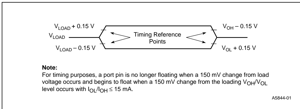
Figure 13. Float Waveforms
