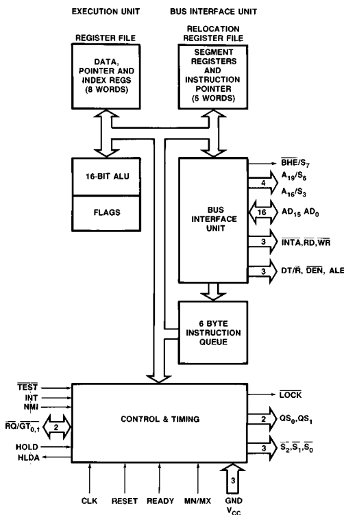
Figure 1. M80C86 CPU Block Diagram
