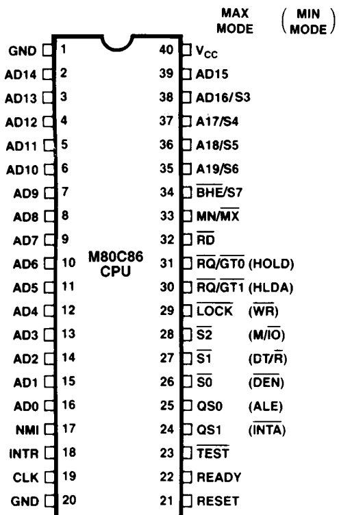
Figure 2. M80C86 40-Lead DIP Configuration
