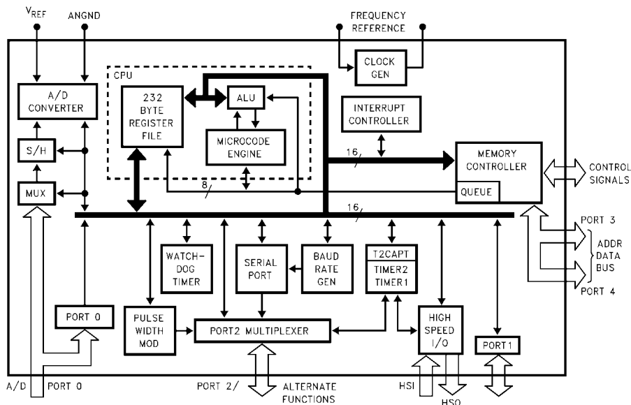
Figure 1. M80C196KB Block Diagram
