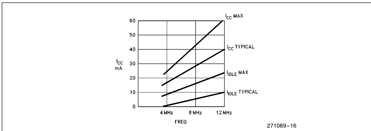
Figure 4. I_{CC} and I_{IDLE} vs Frequency
