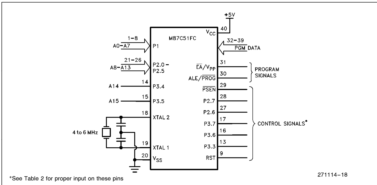
Figure 10. Programming the EPROM
