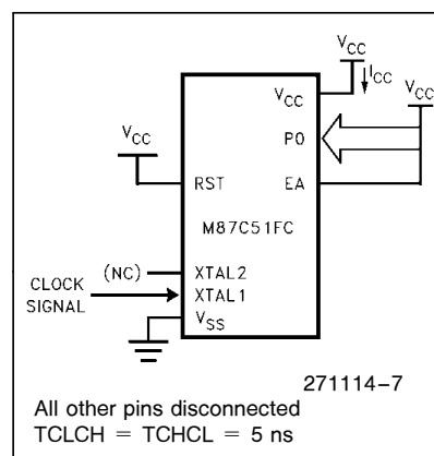
Figure 6. I CC Load Circuits, Active Mode
