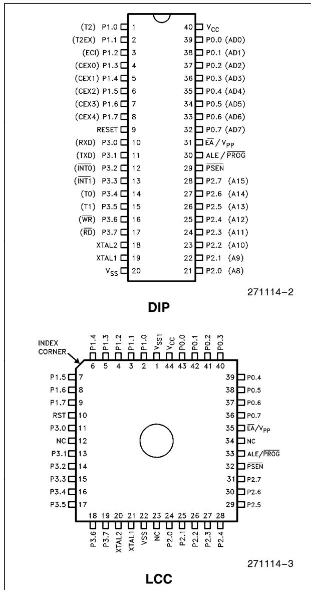
Figure 2. Pin Connections
