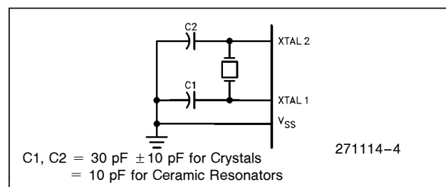
Figure 3. Oscillator Connections
