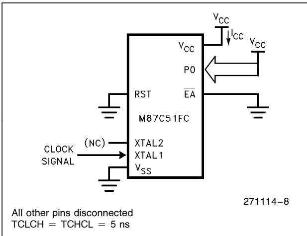
Figure 7. I_{CC} Load Circuit Idle Mode
