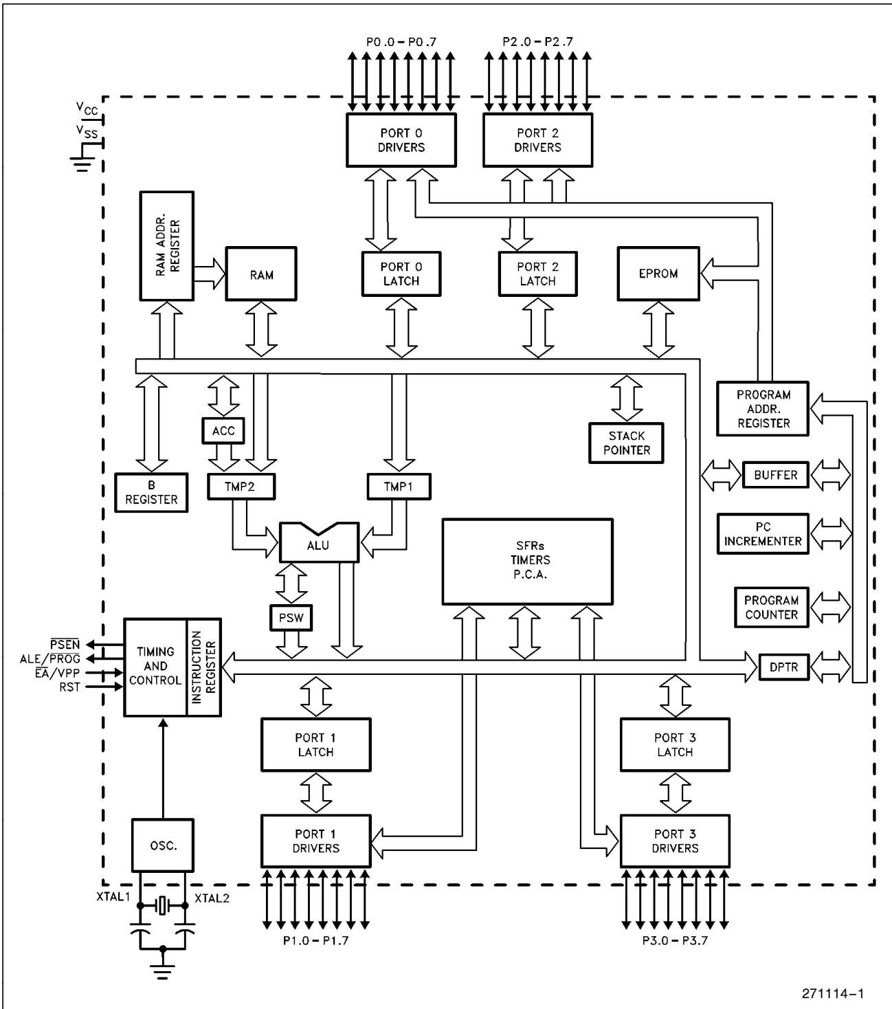
Figure 1. M87C51FC Block Diagram
