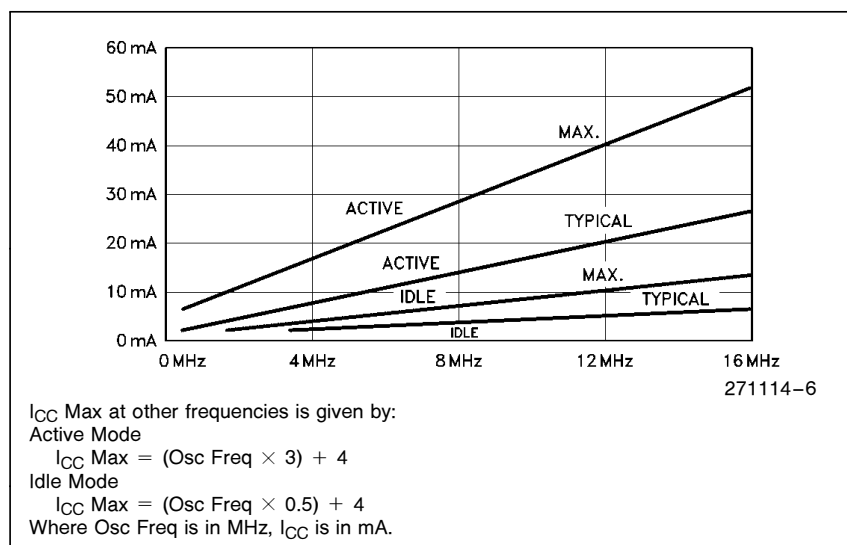
Figure 5. I CC vs Frequency
