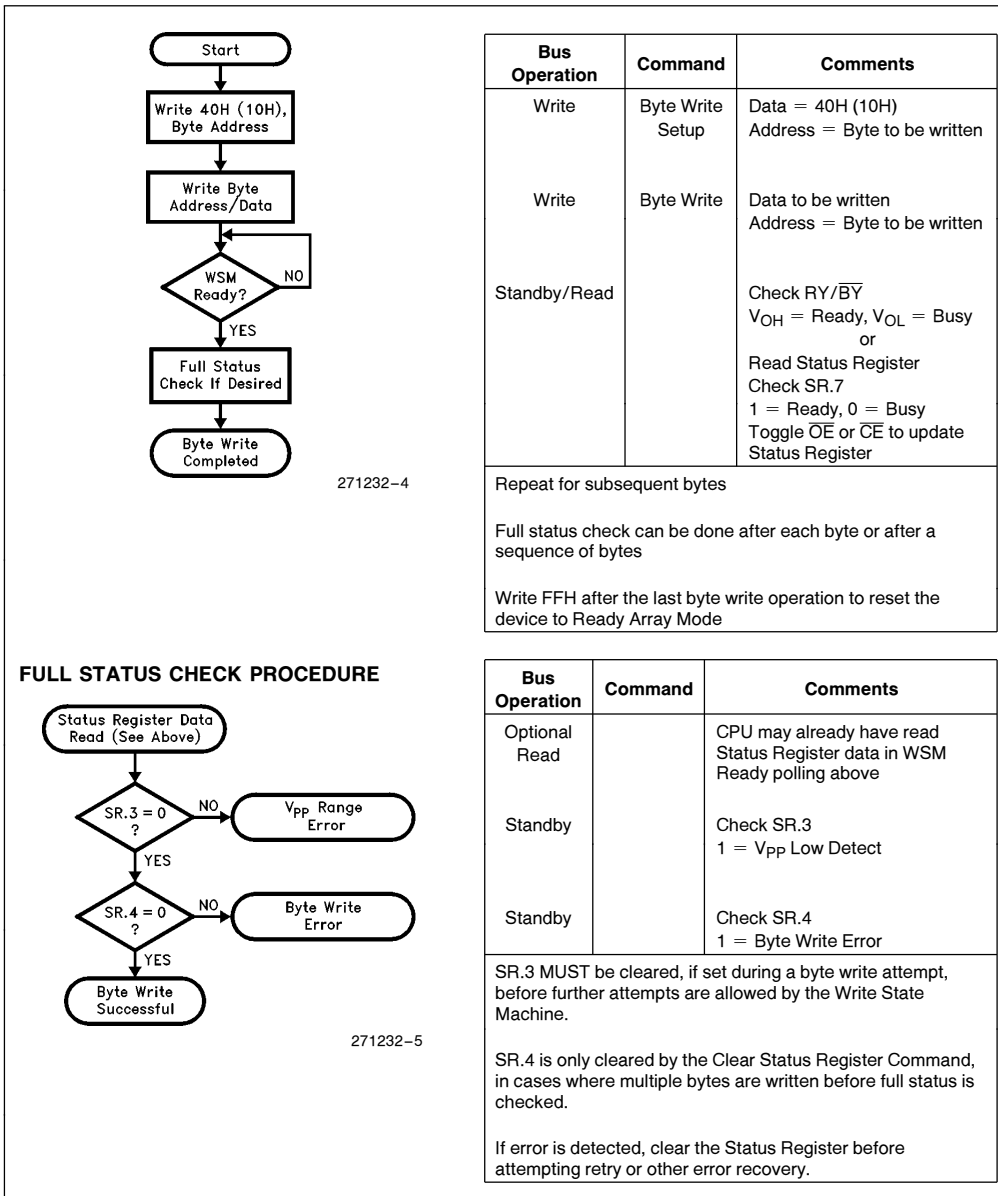
Figure 5. Automated Byte Write Flowchart
