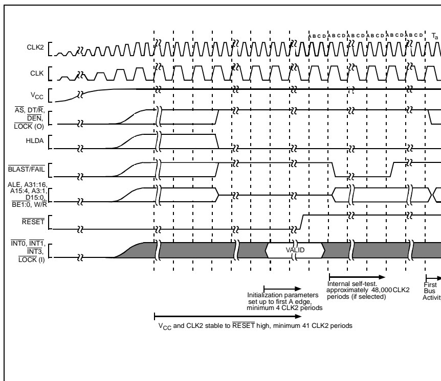
Figure 22. Cold Reset Waveform
