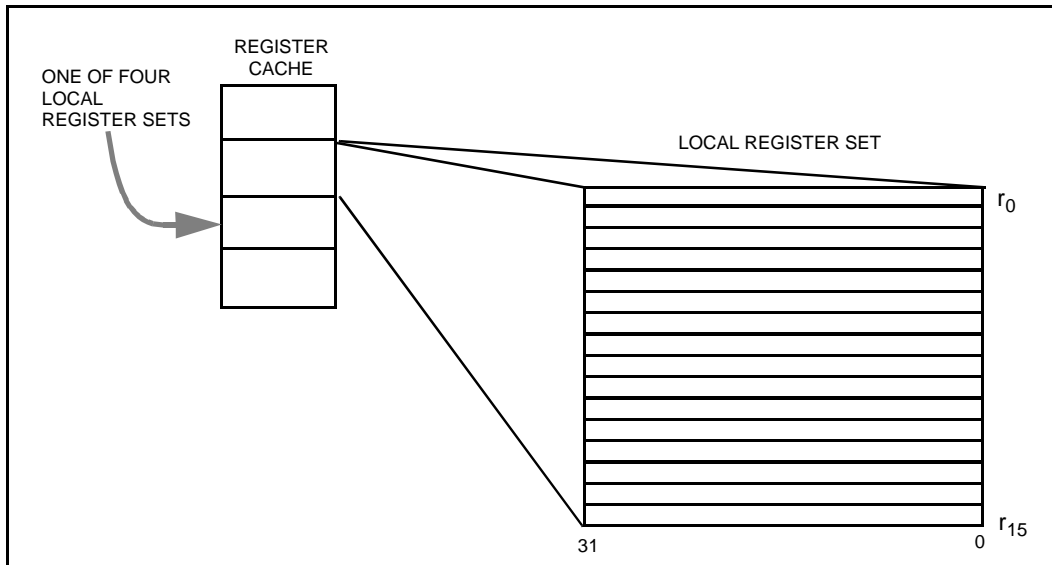
Figure 4. Multiple Register Sets Are Stored On-Chip
