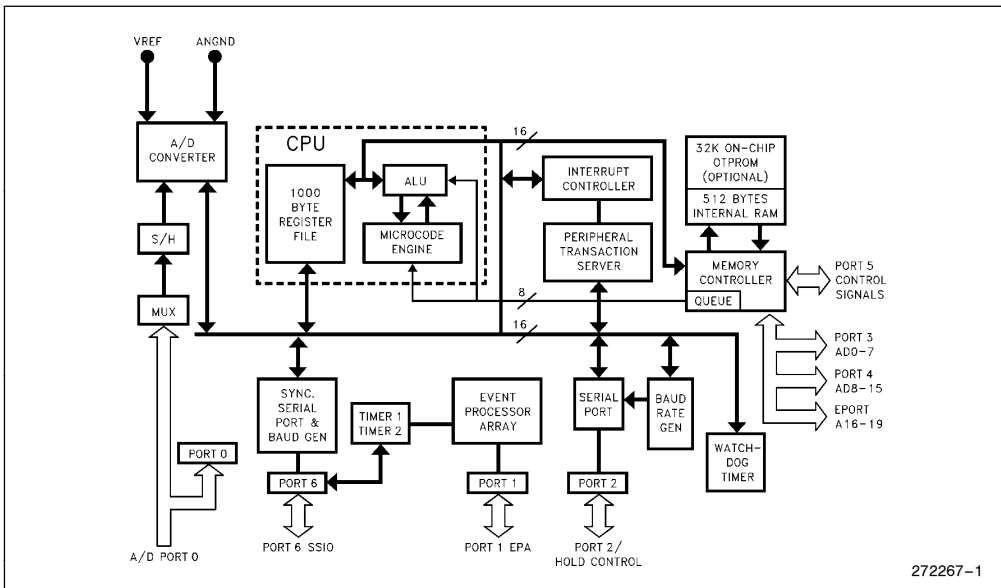
Figure 1. 8XC196NT Block Diagram
