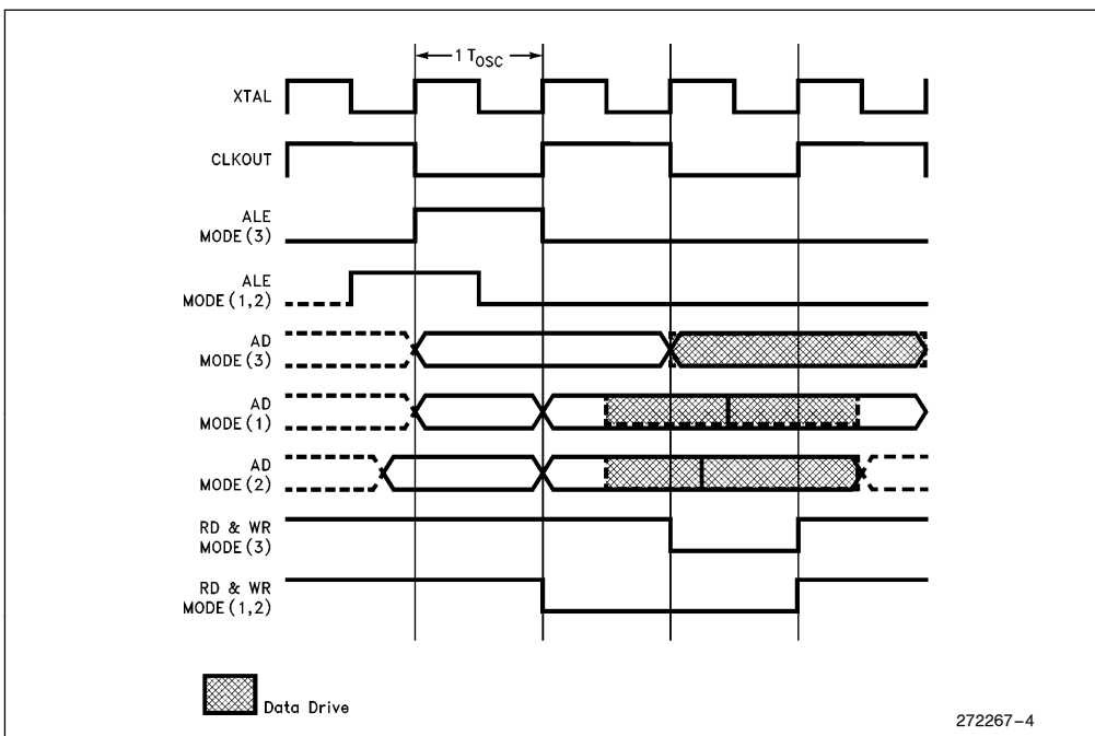
Figure 4. Detailed MODE 1, 2, 3, Comparison
