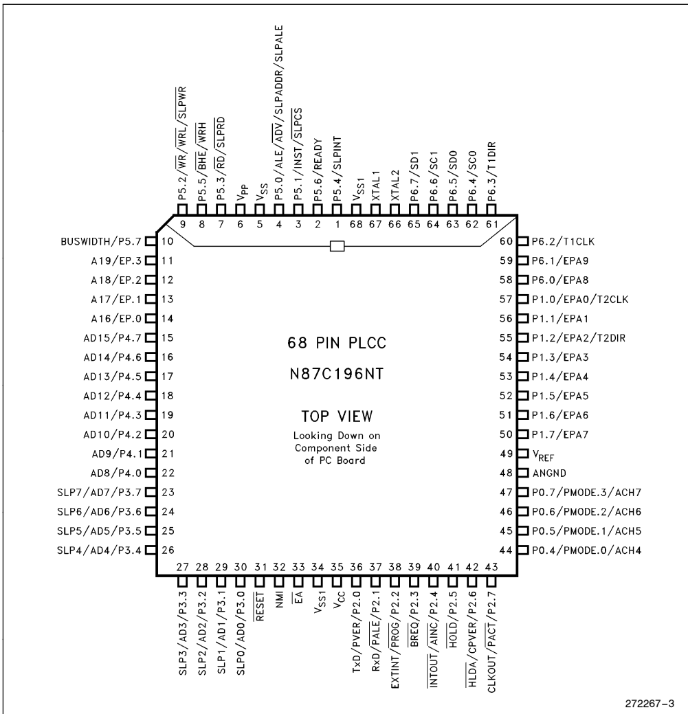
Figure 3. 68-Pin PLCC Package Diagram
