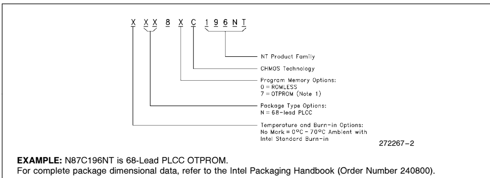
Figure 2. The 8XC186NT Family Nomenclature
