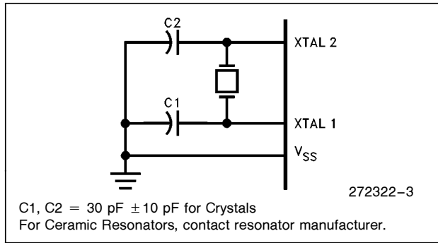
Figure 3. Oscillator Connections
