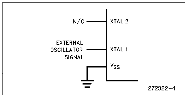
Figure 4. External Clock Drive Configuration
