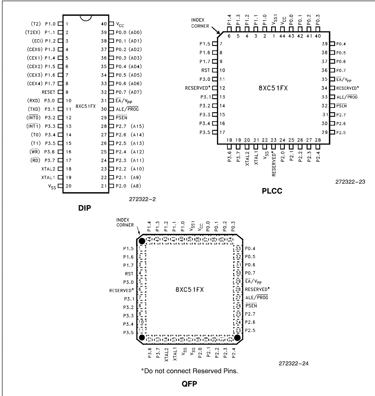
Figure 2. Pin Connections
