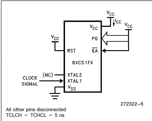
Figure 6. I CC Test Condition, Active Mode
