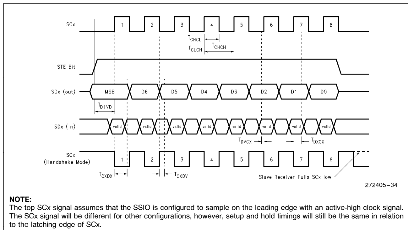
Figure 6. Synchronous Serial Port
