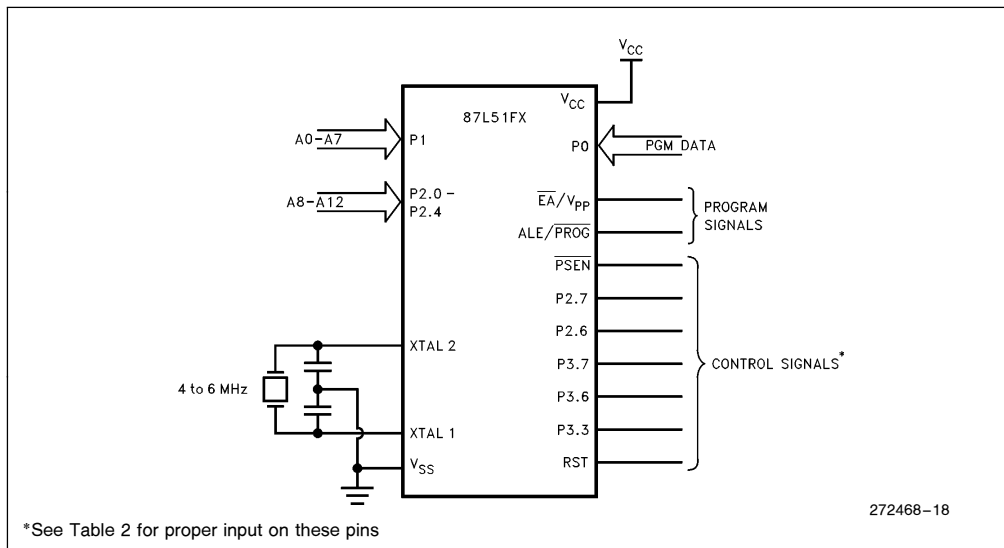
Figure 10. Programming the OTP ROM
