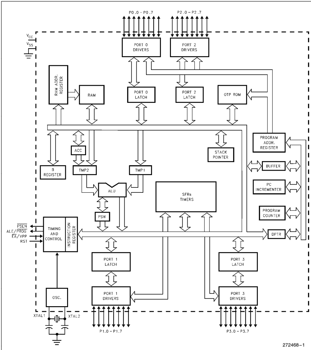
Figure 1. 8XL5X Block Diagram
