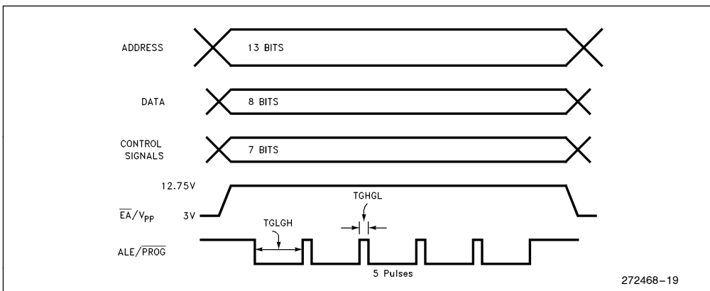
Figure 11. Programming Signals Waveforms
