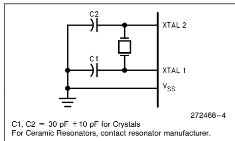
Figure 3. Oscillator Connections
