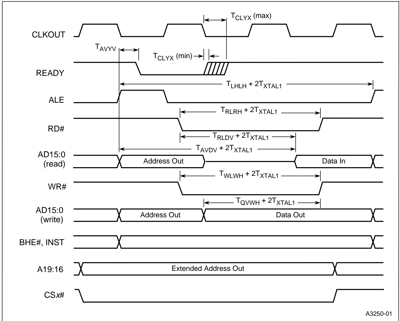
Figure 7. READY Timing Diagram (Multiplexed Bus Mode)
