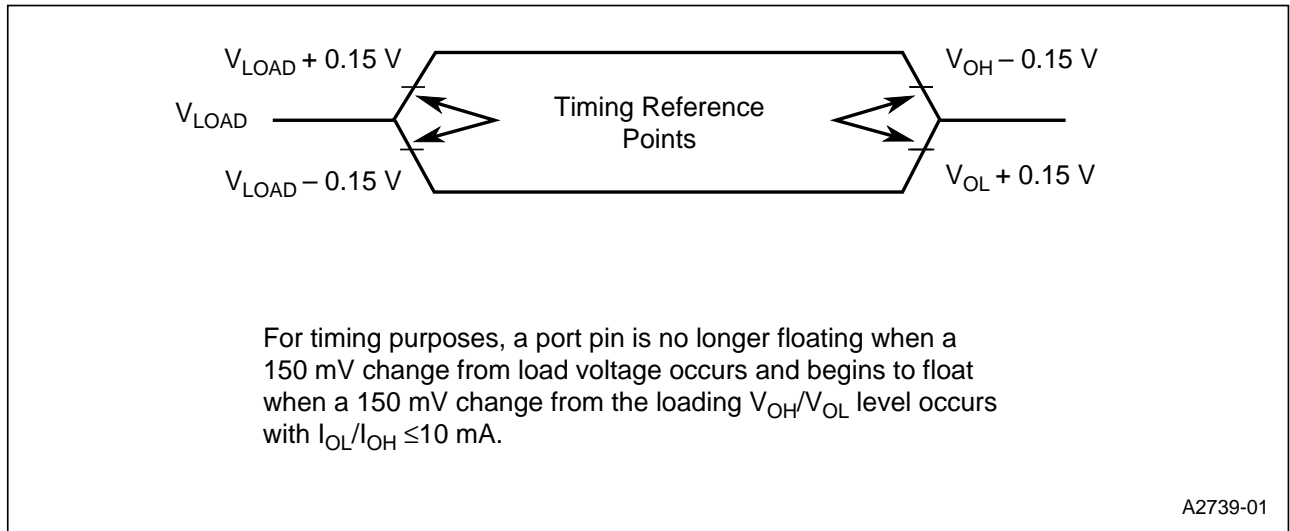
Figure 14. Float Waveforms During 3.0 Volt Testing
