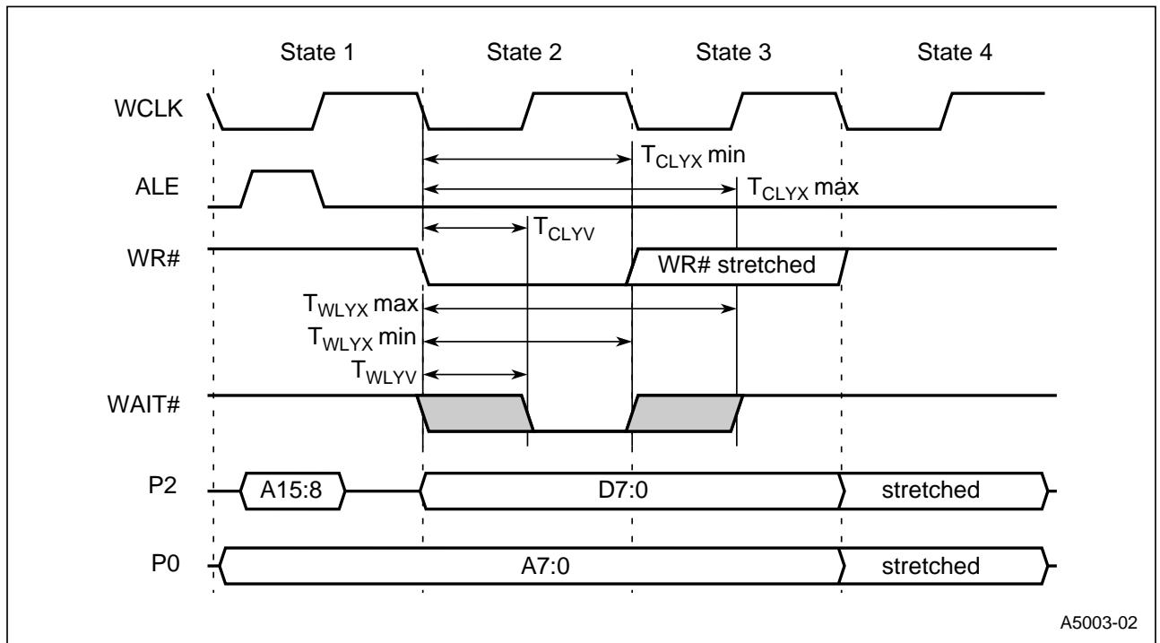
Figure 14. External Bus Cycle: Data Write (Page Mode)
