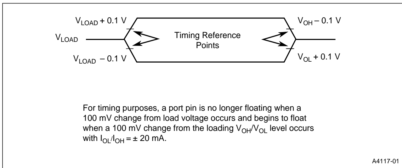
Figure 18. Float Waveforms
