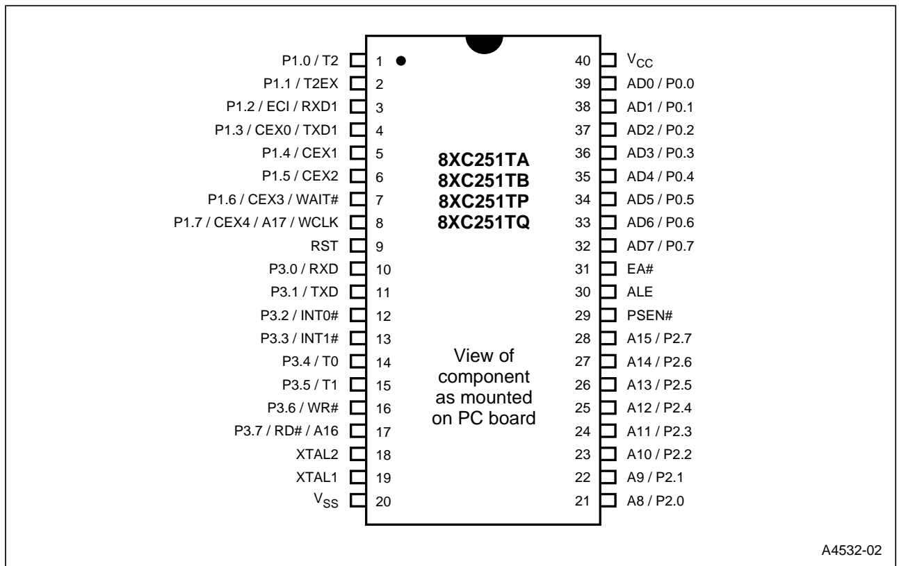
Figure 4. 8xC251TA/TB/TP/TQ 40-pin PDIP Packages
