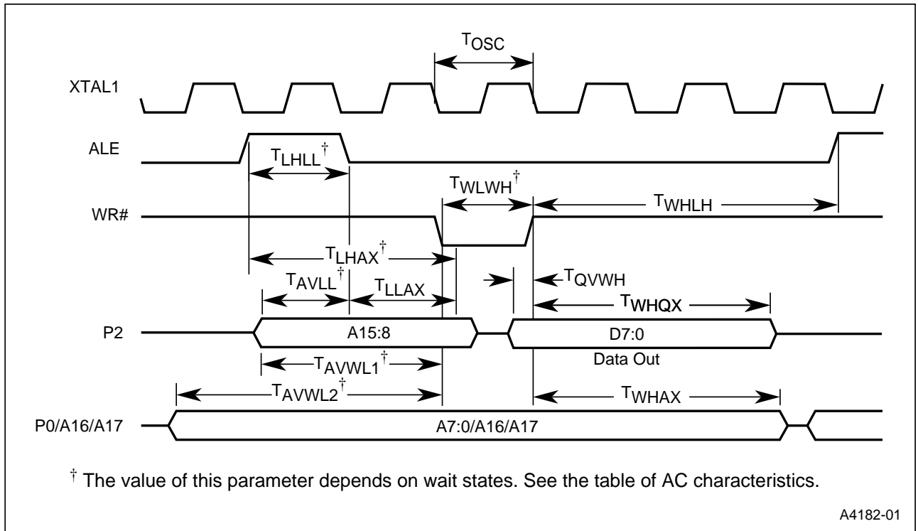
Figure 10. External Bus Cycle: Data Write (Page Mode)
