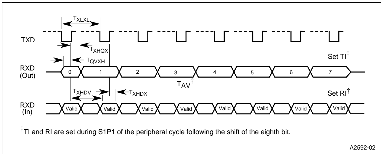
Figure 15. Serial Port Waveform — Shift Register Mode
