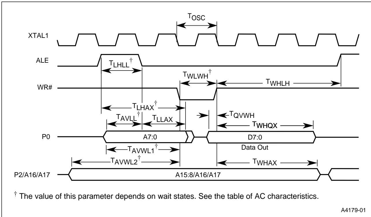
Figure 7. External Bus Cycle: Data Write (Nonpage Mode)
