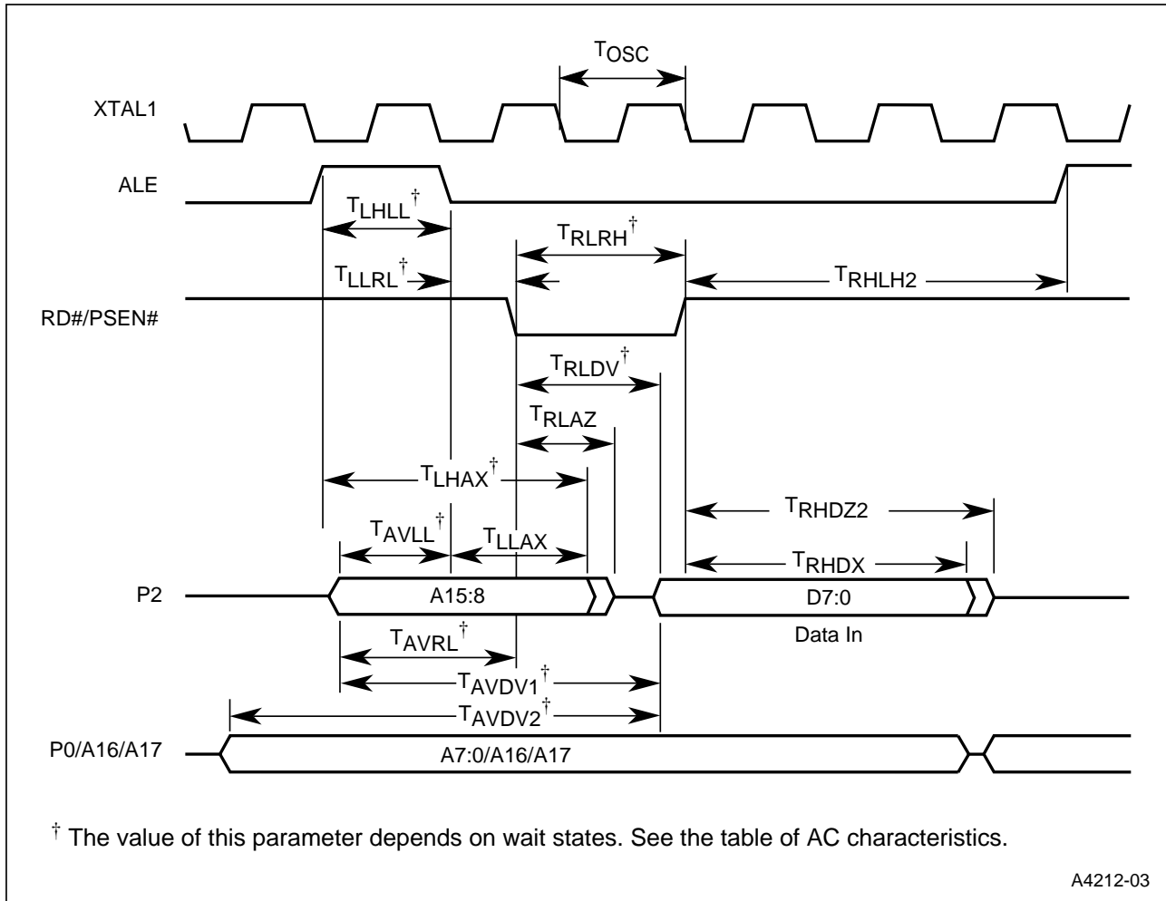
Figure 9. External Bus Cycle: Data Read (Page Mode)
