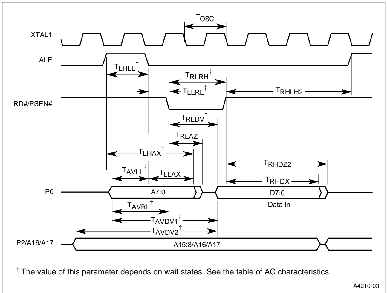
Figure 6. External Bus Cycle: Data Read (Nonpage Mode)
