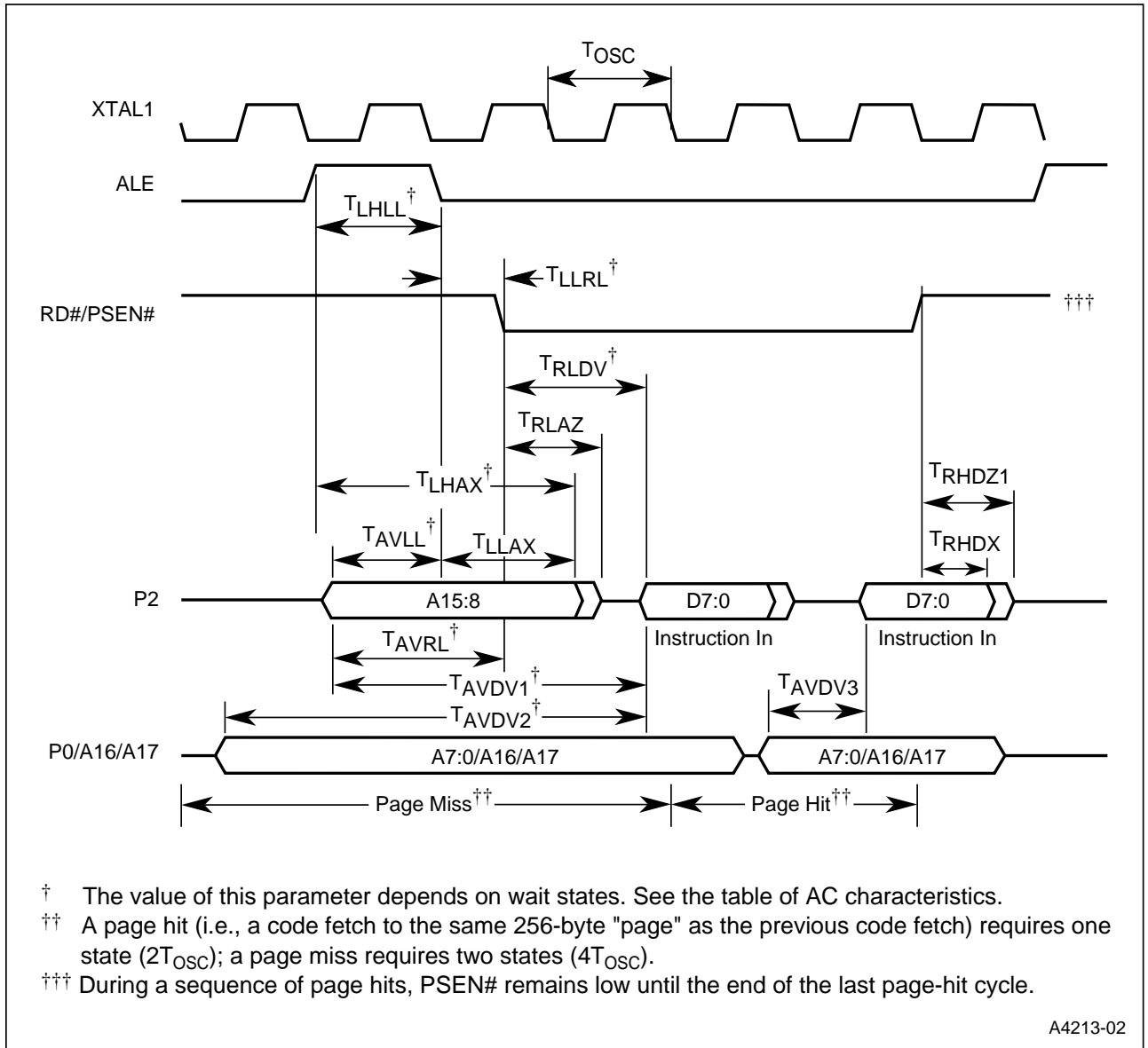
Figure 8. External Bus Cycle: Code Fetch (Page Mode)
