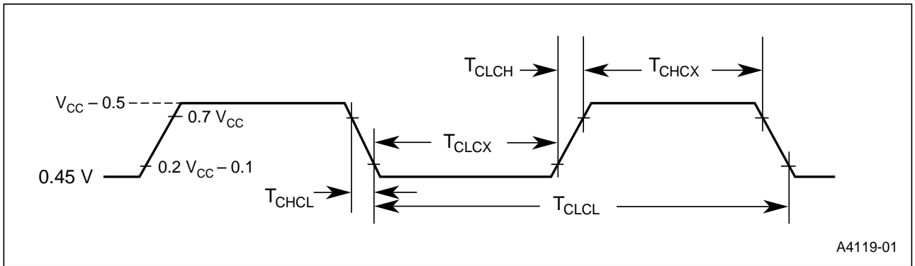
Figure 16. External Clock Drive Waveforms
