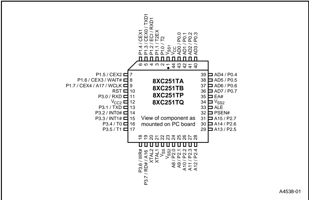
Figure 3. 8xC251TA/TB/TP/TQ 44-pin PLCC Package
