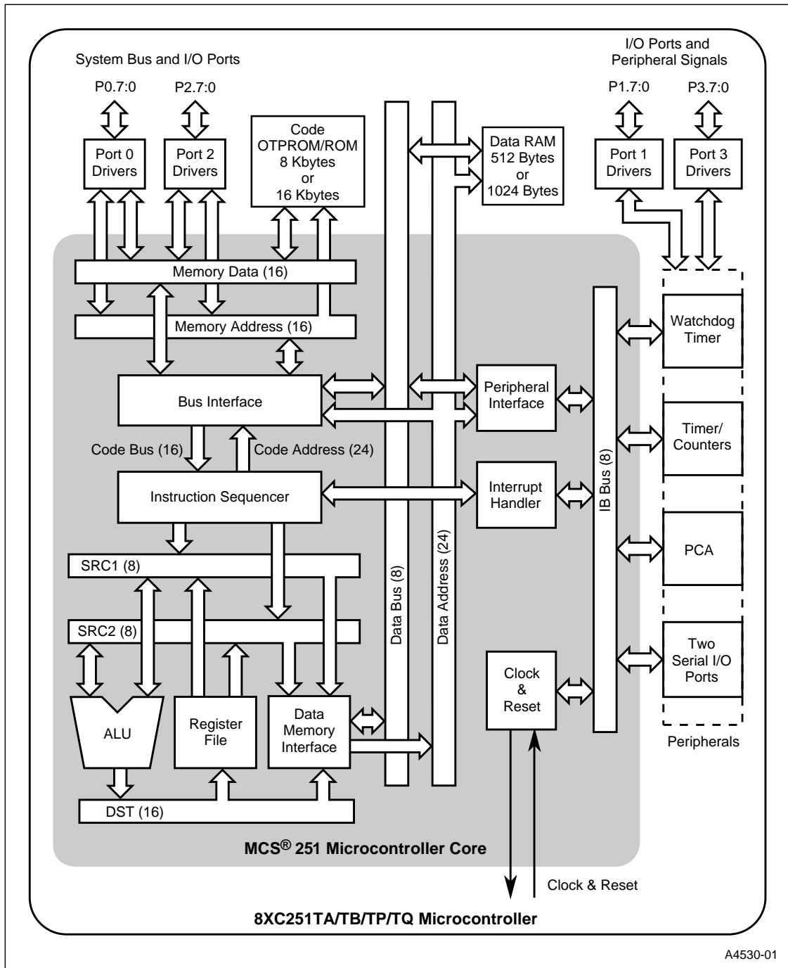
Figure 1. 8xC251TA/TB/TP/TQ Block Diagram
