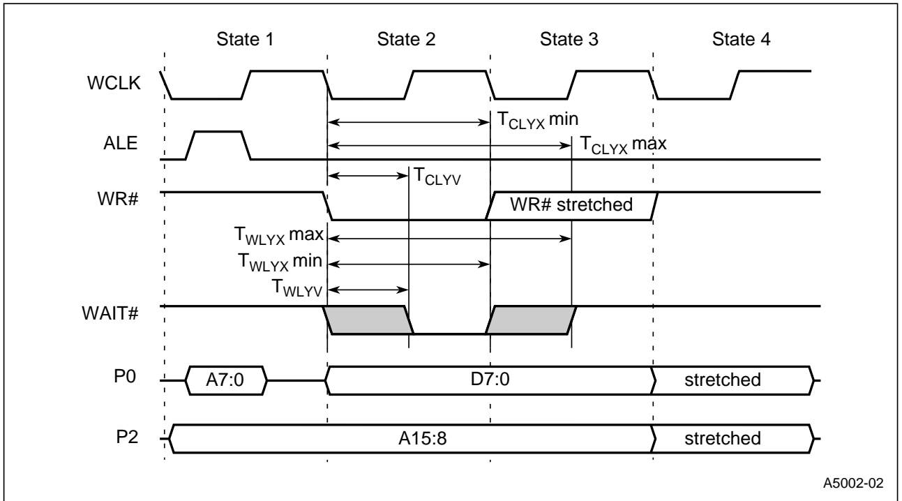
Figure 12. External Bus Cycle: Data Write (Nonpage Mode)
