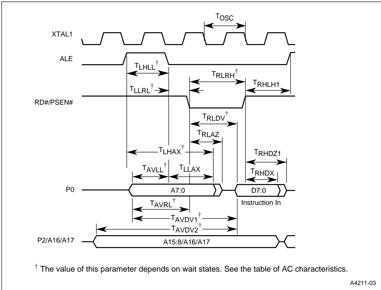
Figure 5. External Bus Cycle: Code Fetch (Nonpage Mode)
