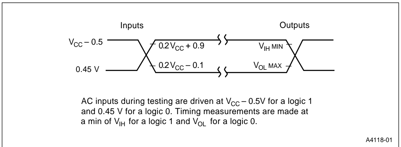
Figure 17. AC Testing Input, Output Waveforms
