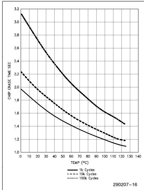
Figure 11. Typical Erase Time at 12V
