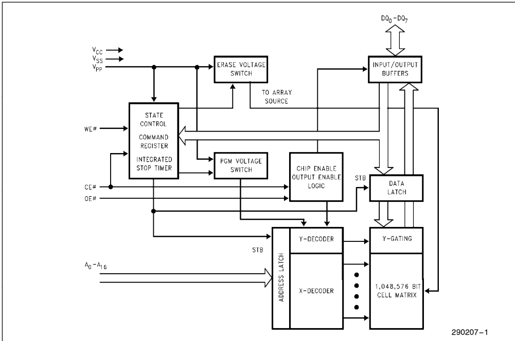
Figure 1. 28F010 Block Diagram
