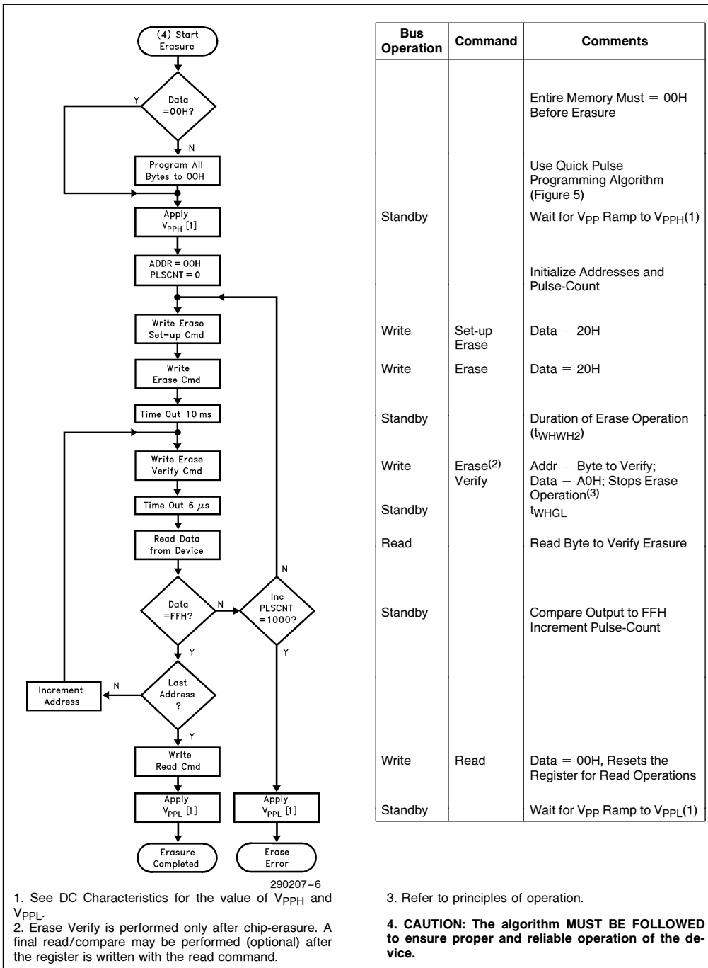
Figure 6. 28F010 Quick Erase Algorithm
