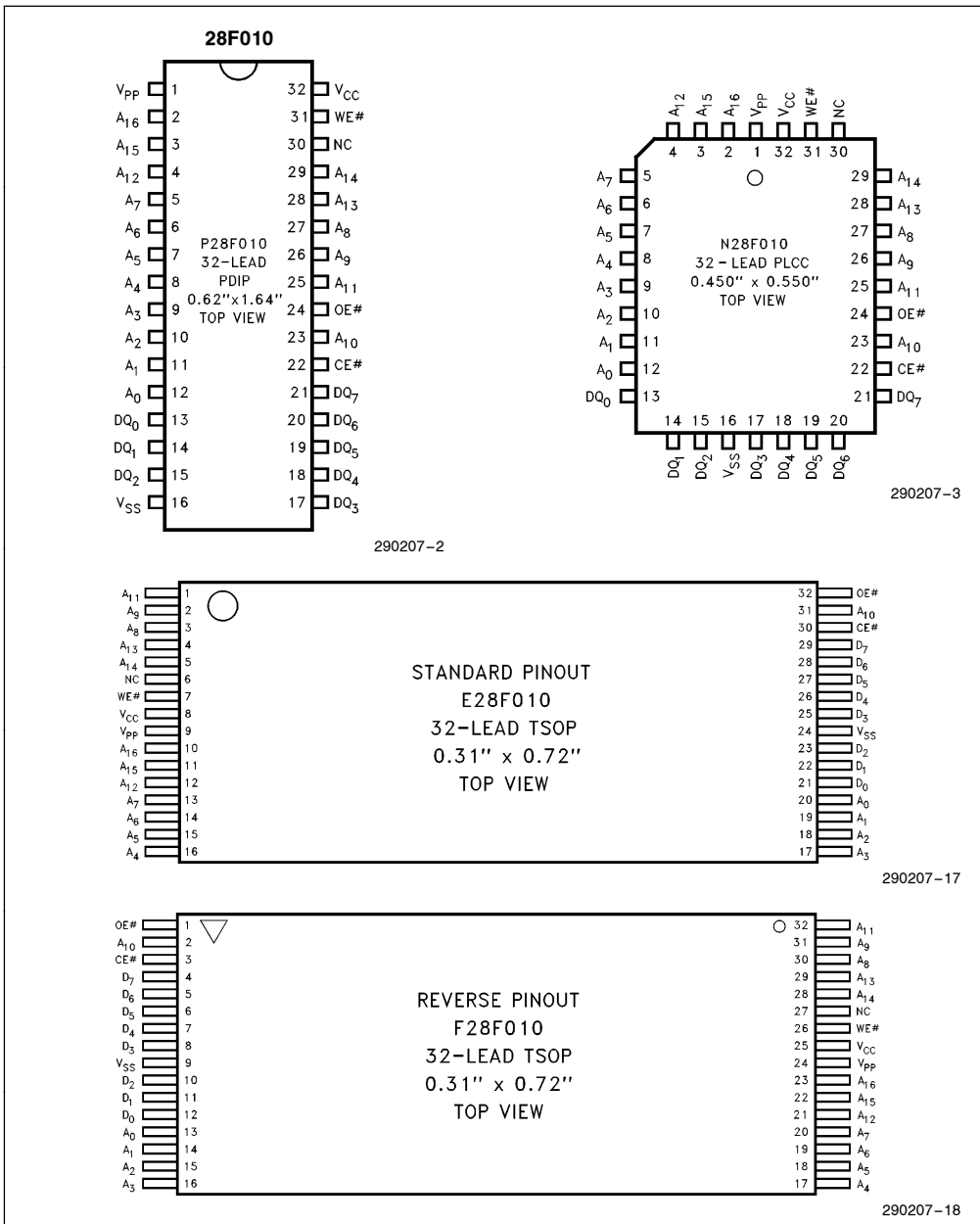
Figure 2. 28F010 Pin Configurations
