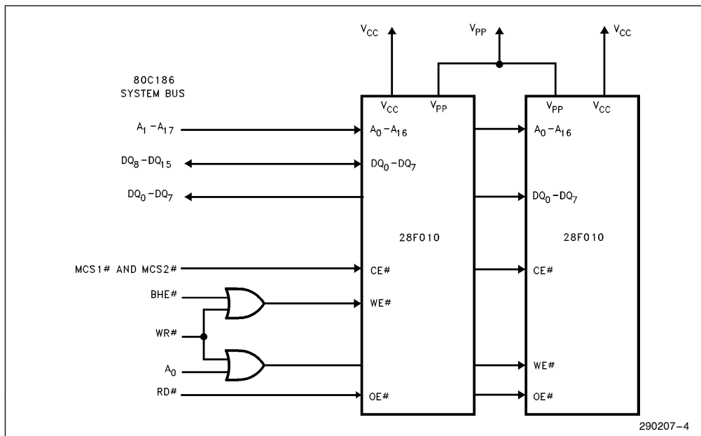
Figure 4. 28F010 in a 80C186 System
