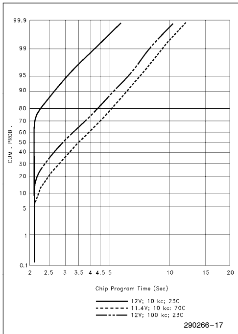
Figure 7. 28F010 Typical Programming Capability See Note 1, Page 18.
