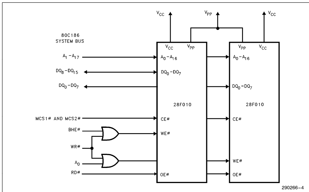
Figure 3. 28F010 in a 80C186 System
