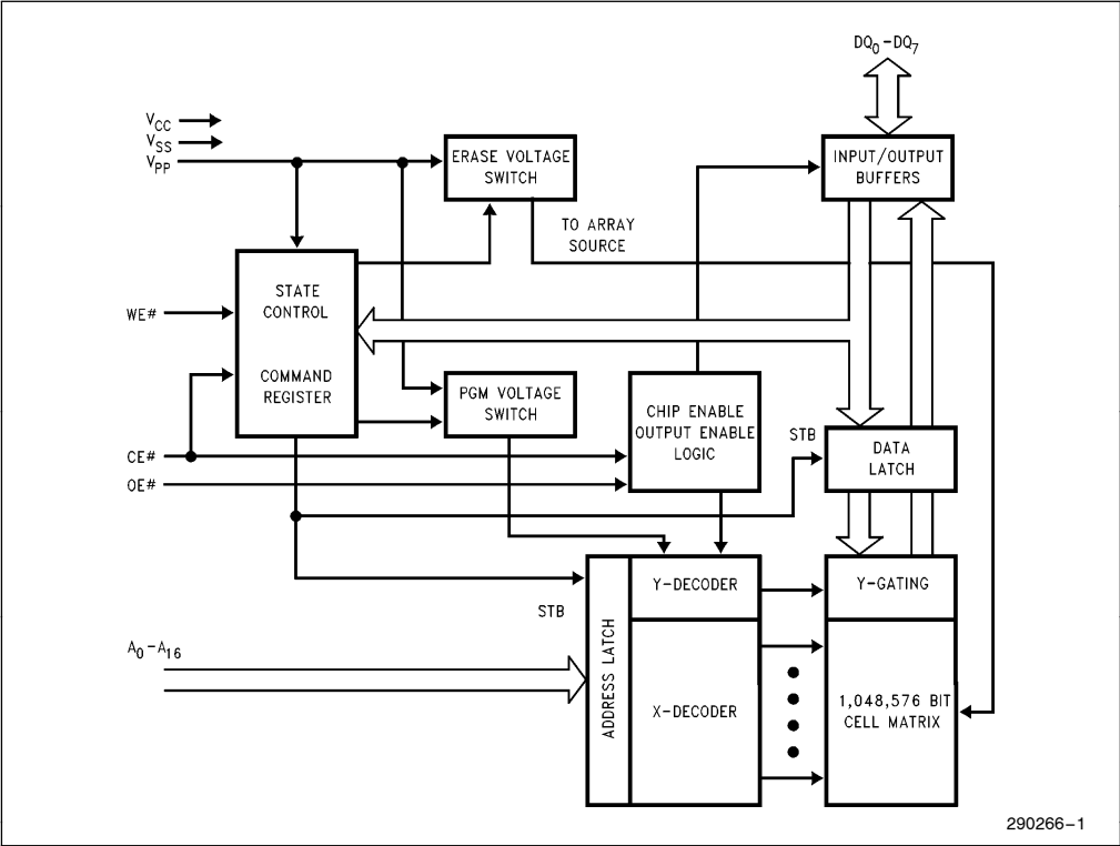
Figure 1. 28F010 Block Diagram
