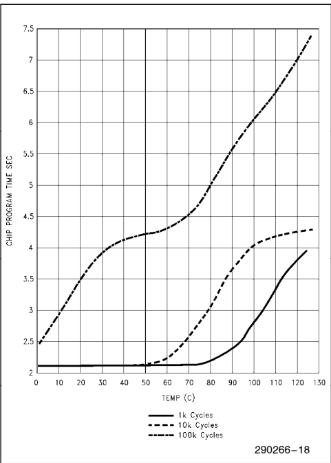
Figure 8. 28F010 Typical Program Time at 12V
