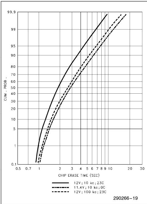
Figure 9. 28F010 Typical Erase Capability See Note 1, Page 18.
