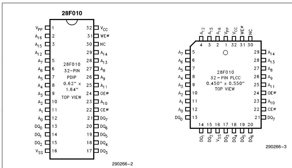
Figure 2. 28F010 Pin Configurations
