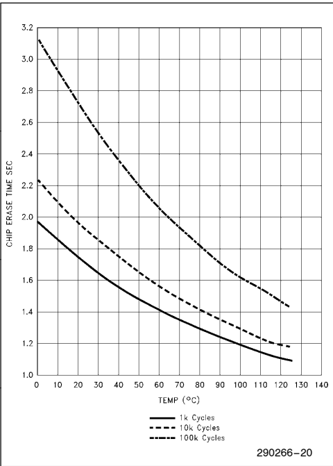
Figure 10. 28F010 Typical Erase Time at 12V
