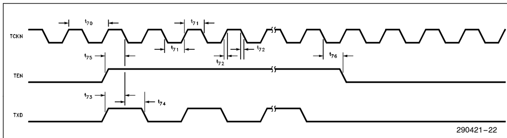
Figure 23. Transmit Timings (Fujitsu)
