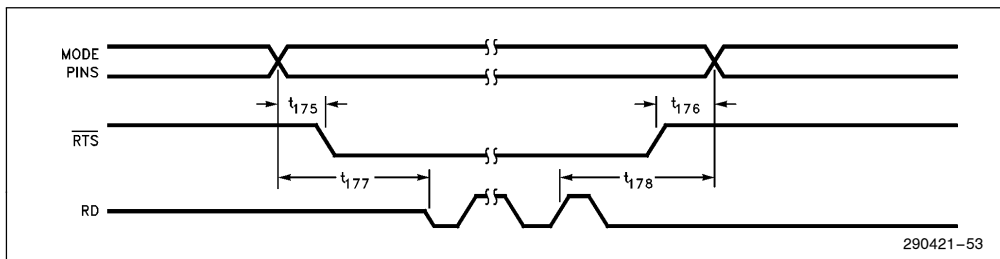
Figure 41. Mode Timings
