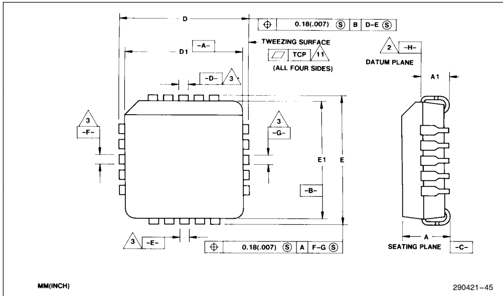
Figure 45. Principle Dimensions and Data
