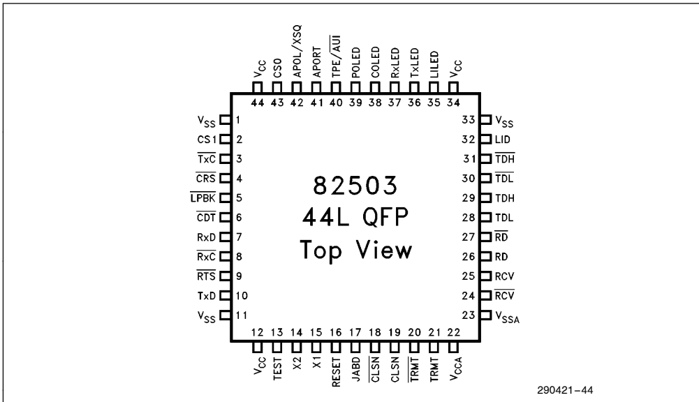
Figure 4. 44-Lead QFP Pin Configuration
