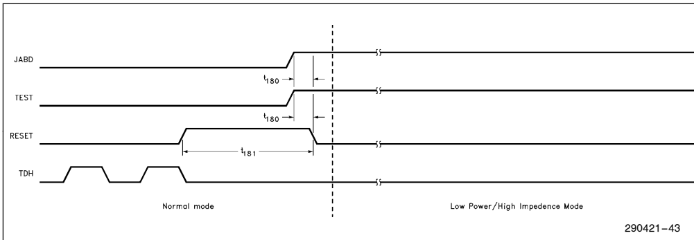
Figure 43. Reset Timings (Start of Low Power Mode)
