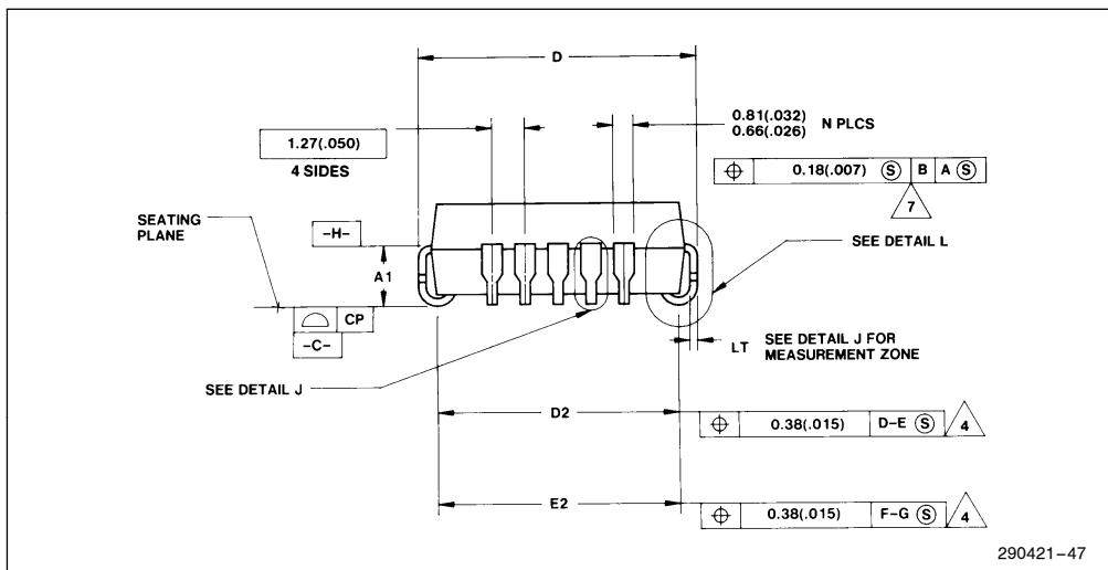
Figure 47. Terminal Details
