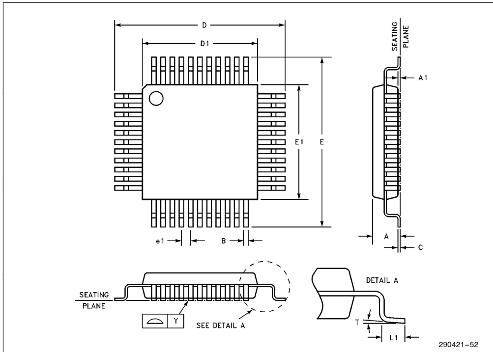
Figure 52. 44-Lead Quad Flatpack Package
