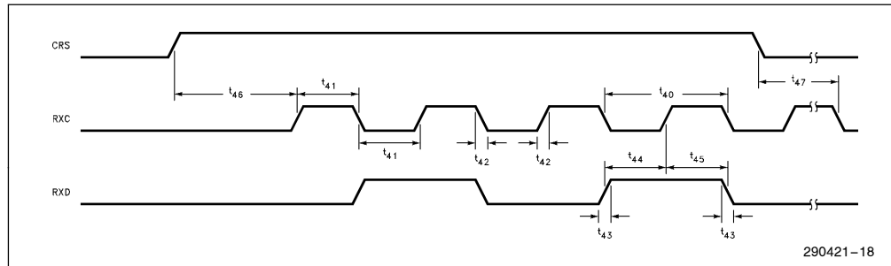
Figure 19. Receiving Timings (National)
