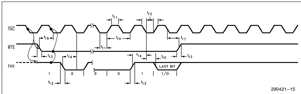
Figure 16. Transmit Timing (Intel)
