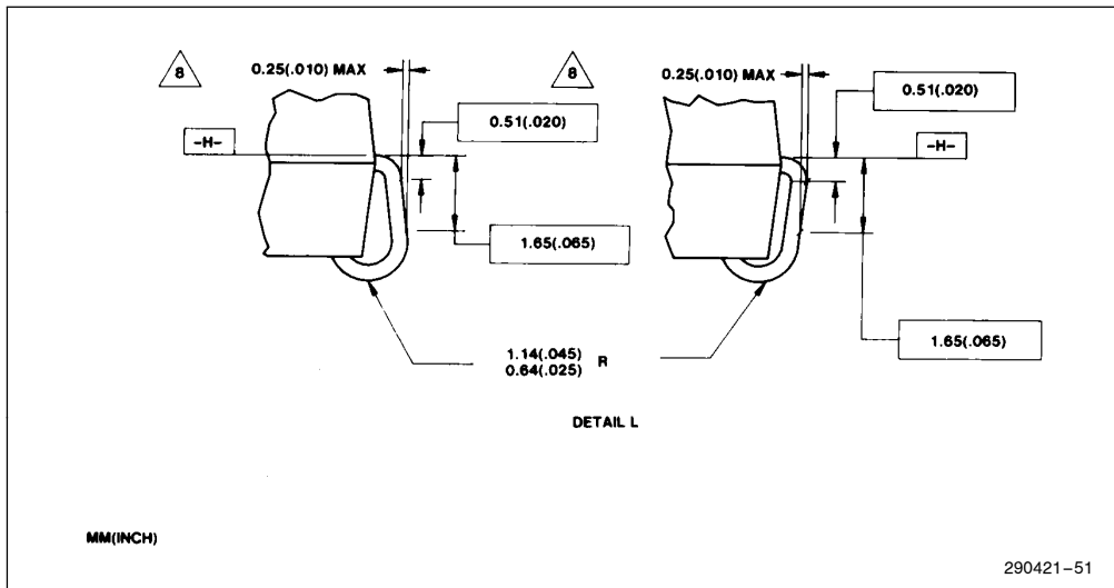
Figure 51. Detail L. Terminal Details
