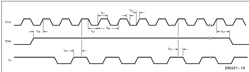
Figure 20. Transmit Timings (AMD)
