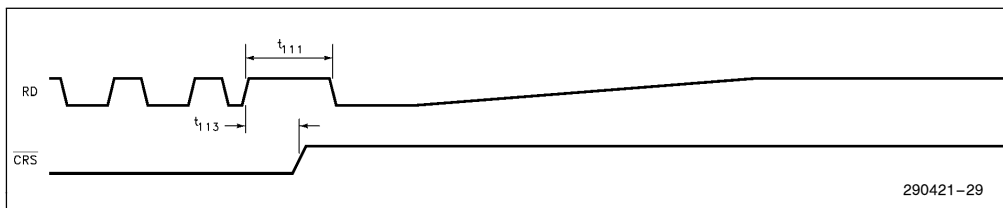
Figure 30. TPE Receive Timings (End of Frame)
