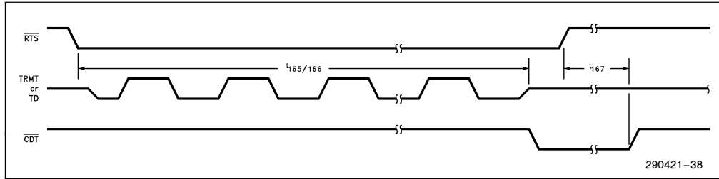
Figure 39. Jabber Timings
