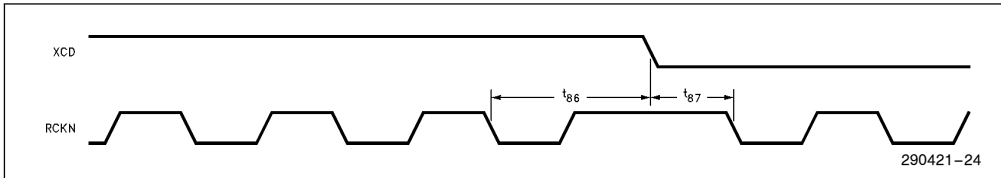
Figure 25. Receive Timings (Fujitsu—End of Frame)
