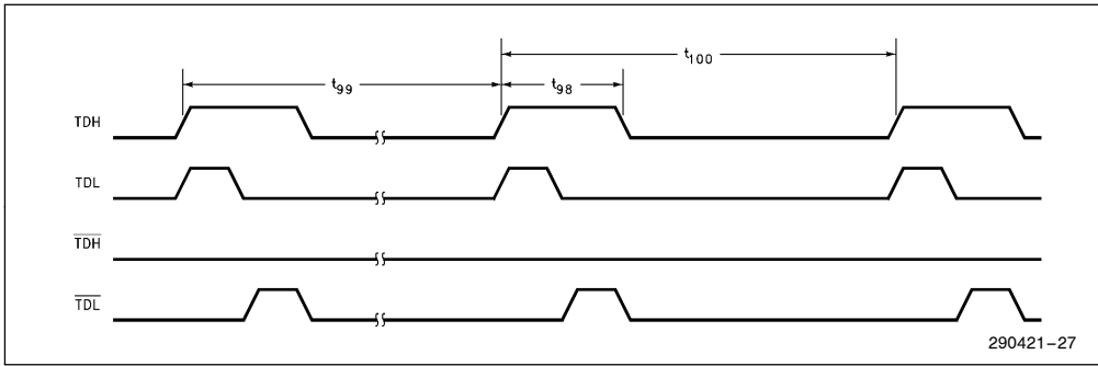
Figure 28. TPE Transmit Timings (Link Test Pulse)
