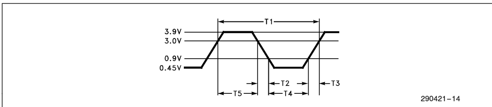
Figure 15. X1 Input Voltage Levels for Timing Measurements
