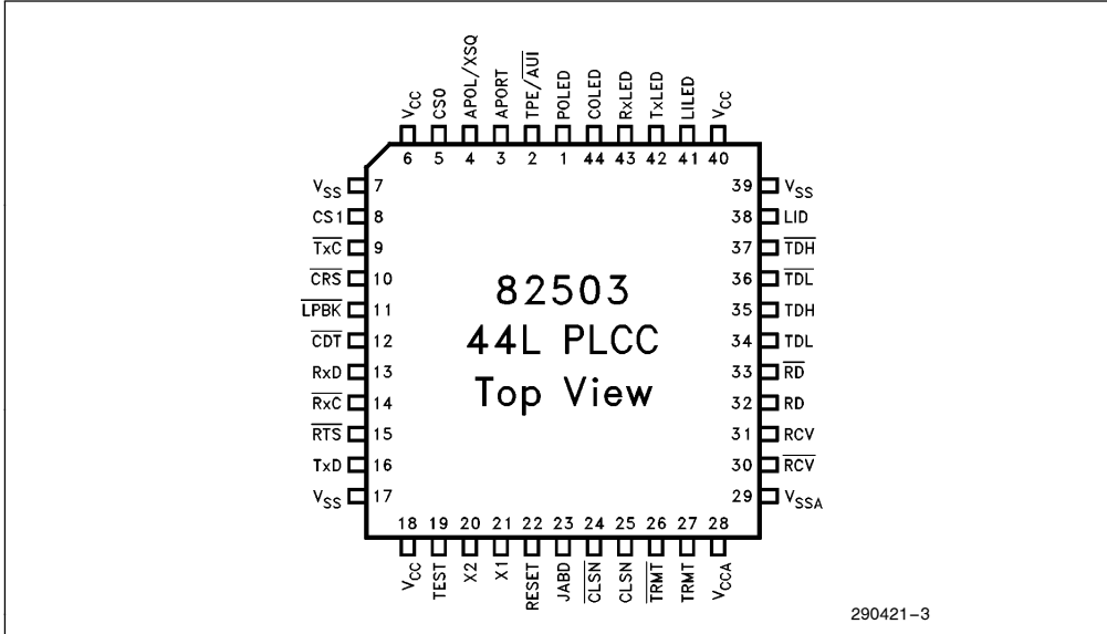
Figure 3. 44-Lead PLCC Pin Configuration
