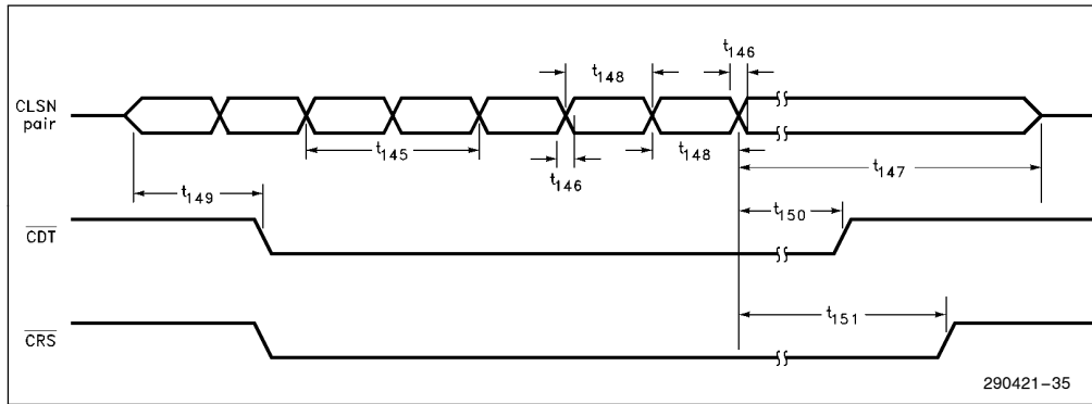
Figure 36. AUI Collision Timings
