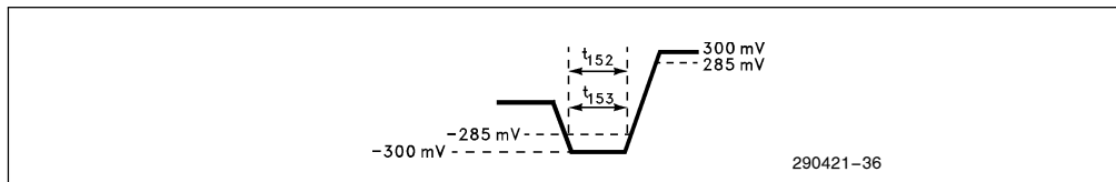
Figure 37. AUI Noise Filter Timings
