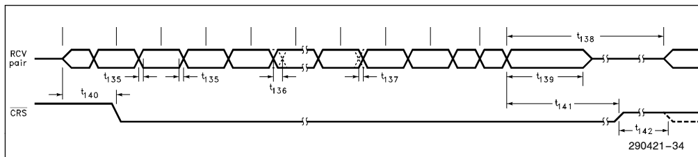
Figure 35. AUI Receive Timings
