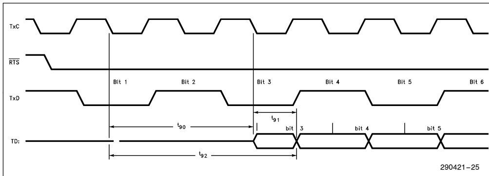
Figure 26. TPE Transmit Timings (Start of Frame)
