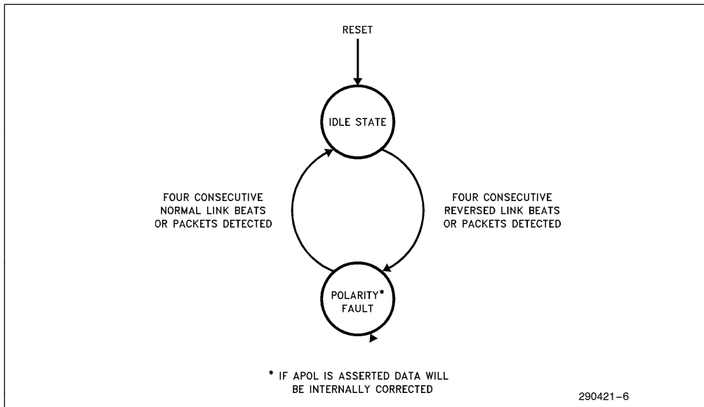
Figure 7. Polarity Fault State Diagram
