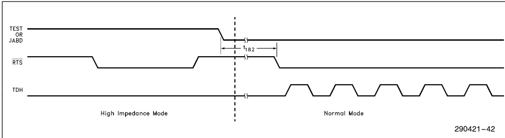
Figure 44. Reset Timings (End of Low Power Mode)
