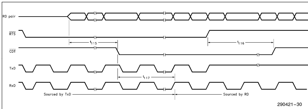
Figure 31. TPE Collision Timings (Start of Collision)
