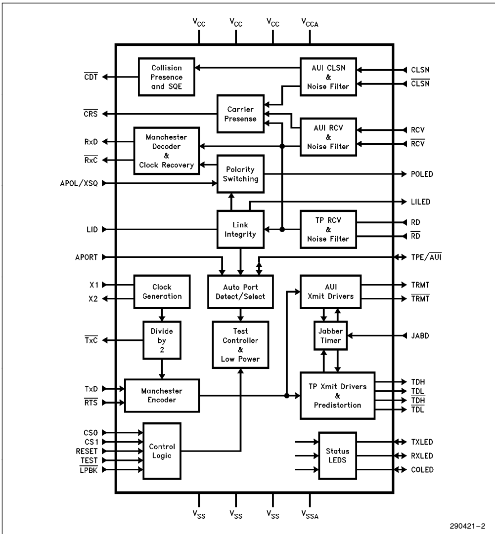
Figure 2. 82503 Functional Block Diagram
