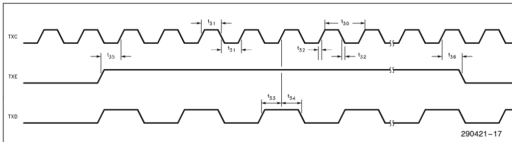
Figure 18. Transmit Timing (National)
