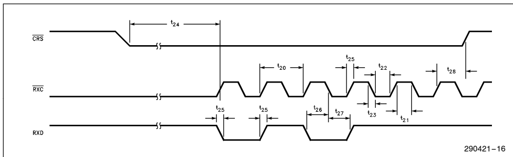
Figure 17. Receive Timing (Intel)
