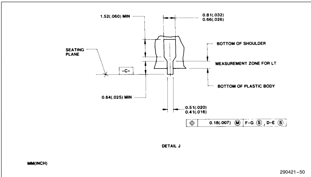
Figure 50. Detail J. Terminal Detail
