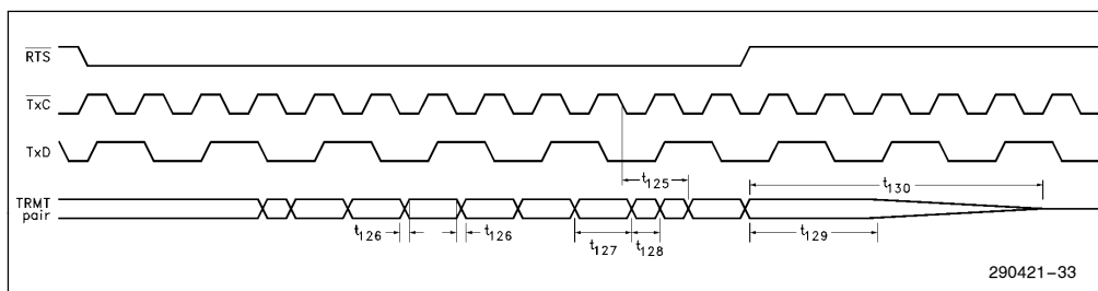
Figure 34. AUI Transmit Timings
