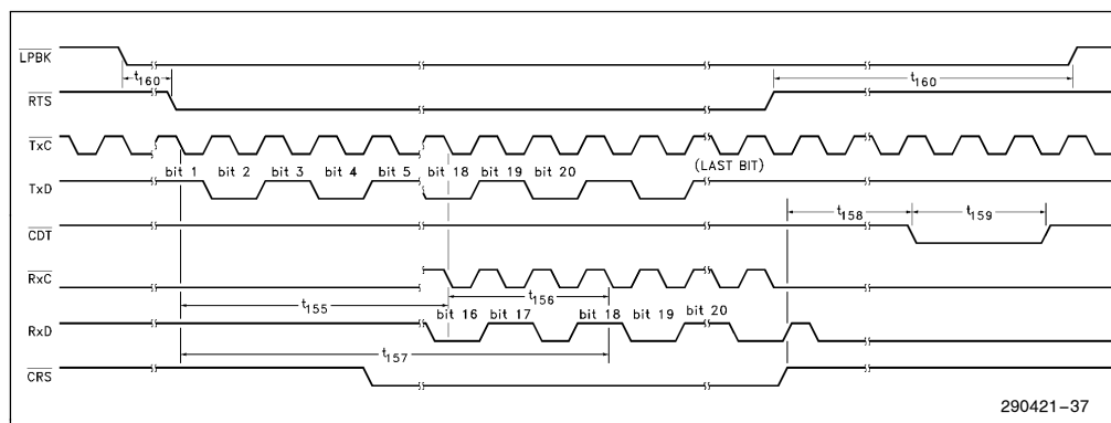
Figure 38. Loopback Timings
