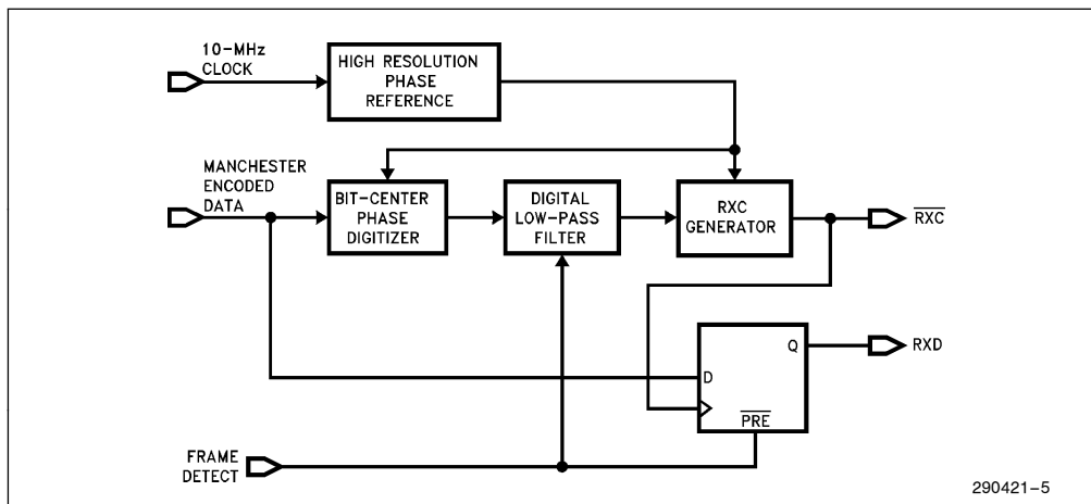
Figure 6. Manchester Decoder and Clock Recovery
