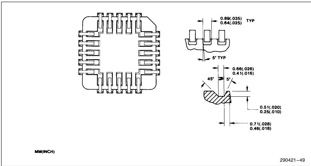
Figure 49. Standard Package Bottom View (Tooling Option II)
