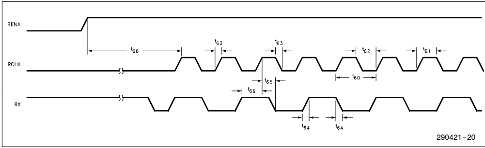
Figure 21. Receive Timings (AMD—Start of Frame)
