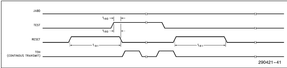
Figure 42. Reset Timings (Test Mode)
