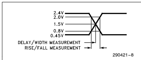
Figure 9. MOS Input Voltage Levels (TTL Compatible) for Timing Measurements (Tx D , \overline{\text{RTS}} , TPE/ \overline{\text{AUI}} , A PORT , APOL/ \overline{\text{XSQ}} , LID, LPBK, JABD, TEST, and RESET).
