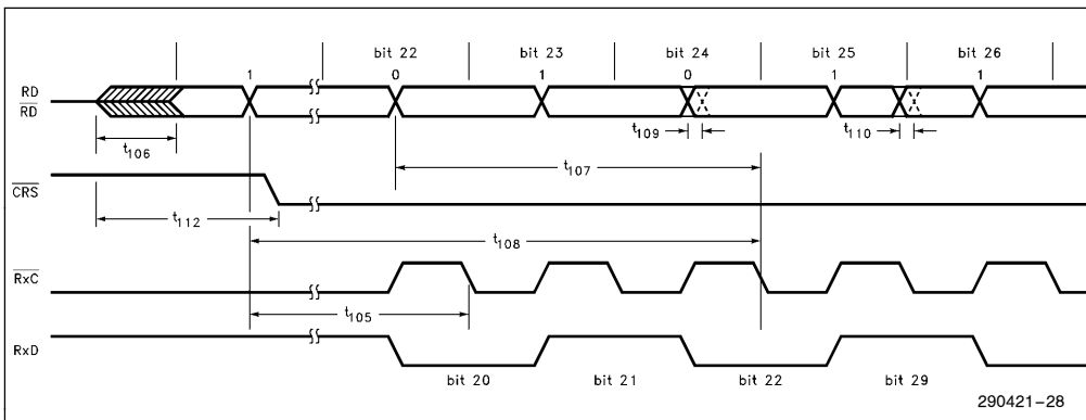
Figure 29. TPE Receive Timings (Start of Frame)
