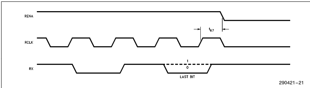
Figure 22. Receive Timings (AMD—End of Frame)
