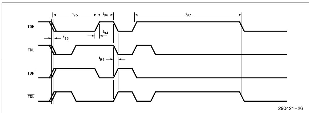
Figure 27. TPE Transmit Timings (End of Frame)
