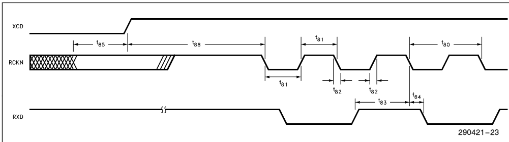
Figure 24. Receive Timings (Fujitsu—Start of Frame)
