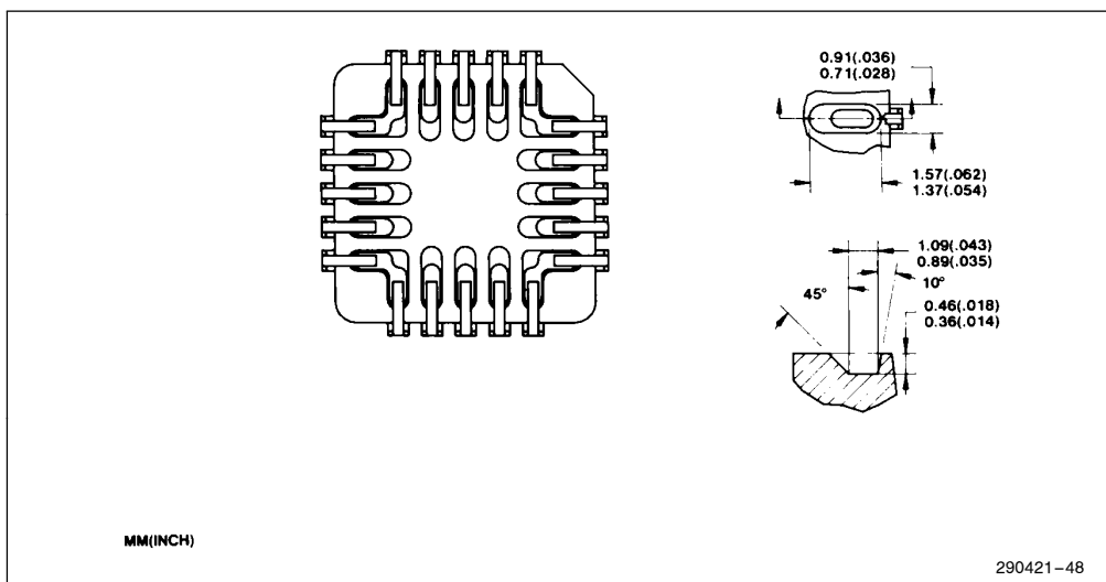
Figure 48. Standard Package Bottom View (Tooling Option 1)
