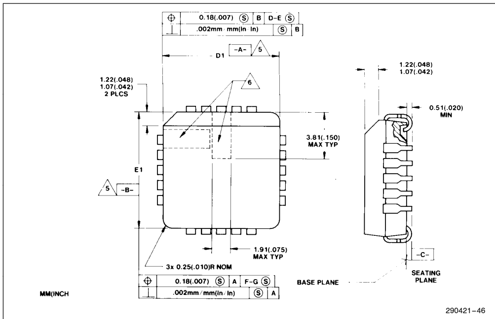
Figure 46. Molded Details
