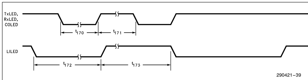
Figure 40. LED Timings
