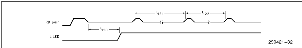
Figure 33. TPE Link Integrity Timings
