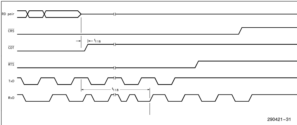
Figure 32. TPE Collision Timings (End of Collision)
