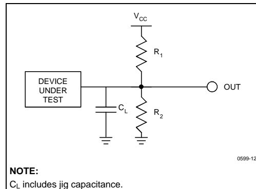
Figure 12. Test Configuration
