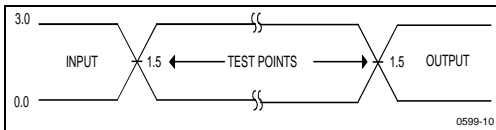
Figure 10. High Speed Test Waveform
