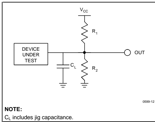
Figure 13. Test Configuration
