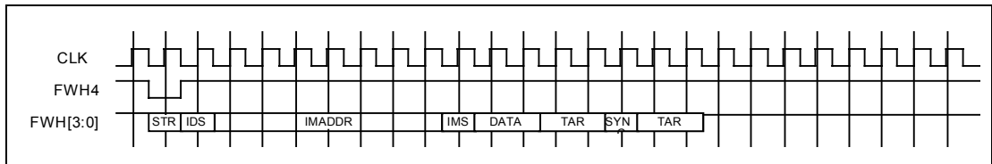
Figure 11. Write Waveforms
