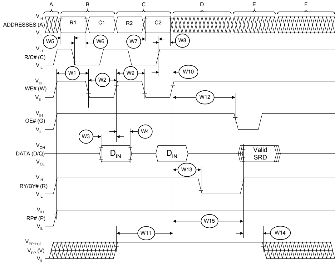
Figure 15. A/A Mux Write Timing Diagram
