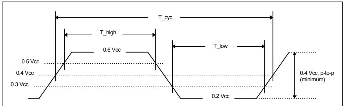
Figure 7. Clock Waveform
