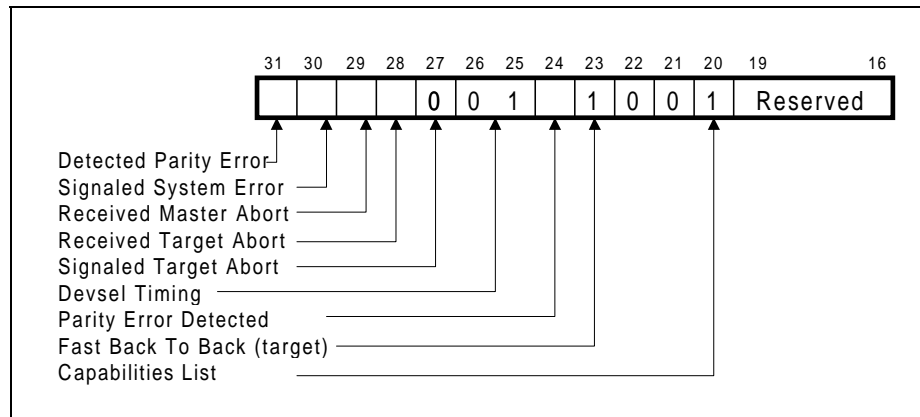
Figure 19. PCI Status Register
