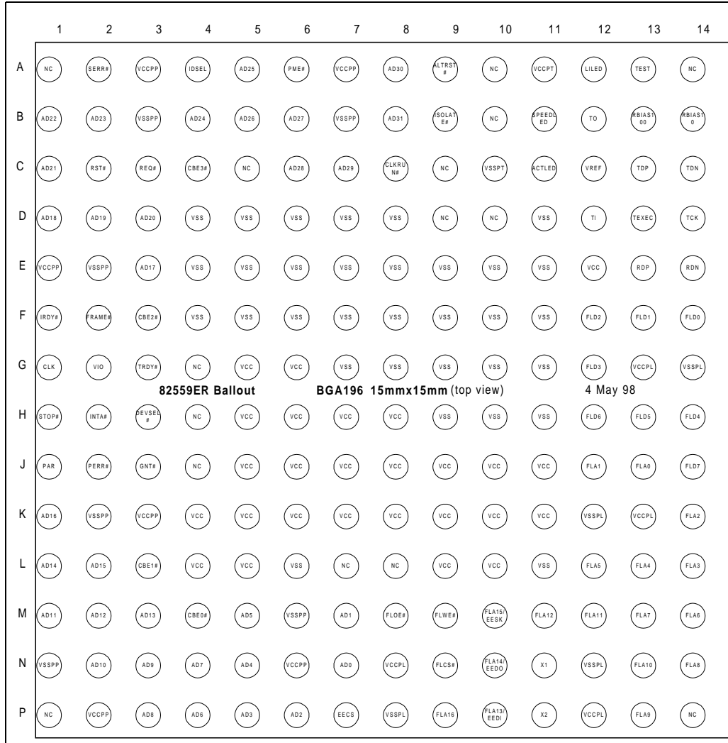
Figure 25. GD82559ER Ball Grid Array Diagram
