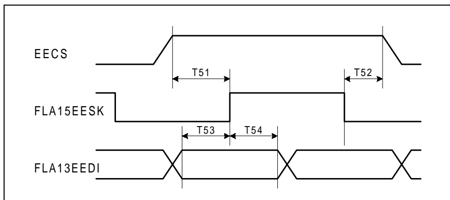
Figure 30. EEPROM Timings
