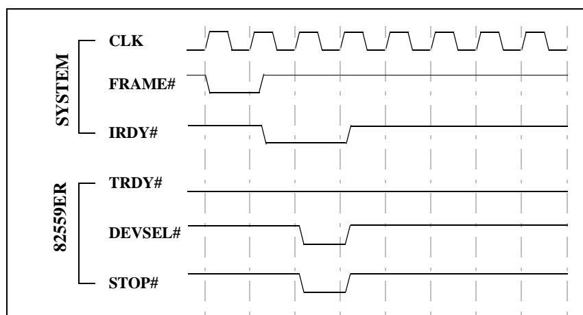
Figure 6. PCI Retry Cycle
