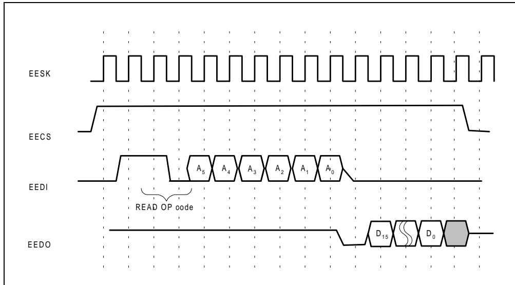
Figure 11. 64 Word EEPROM Read Instruction Waveform
