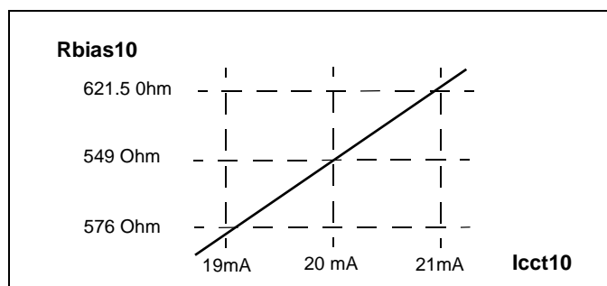
Figure 25. RBIAS10 Resistance Versus Transmitter Current
