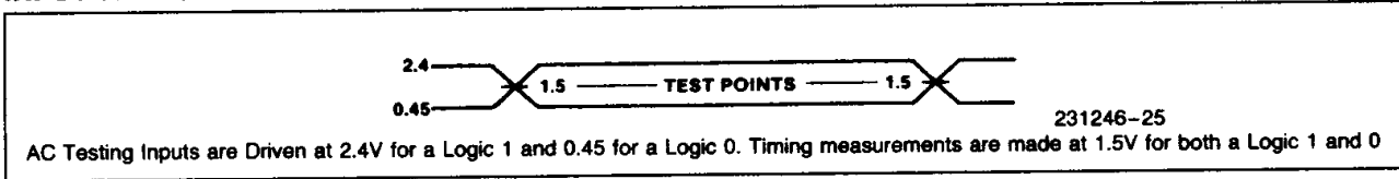
Figure 24. TTL Input/Output Voltage Levels for Timing Measurements
