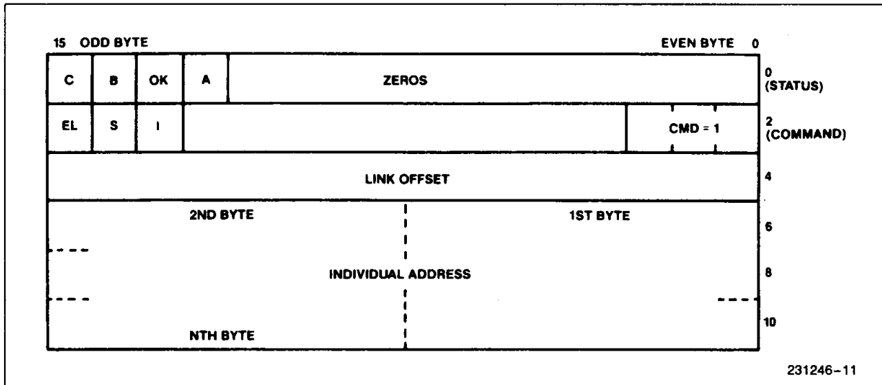
Figure 12. The IA-SETUP Command Block
