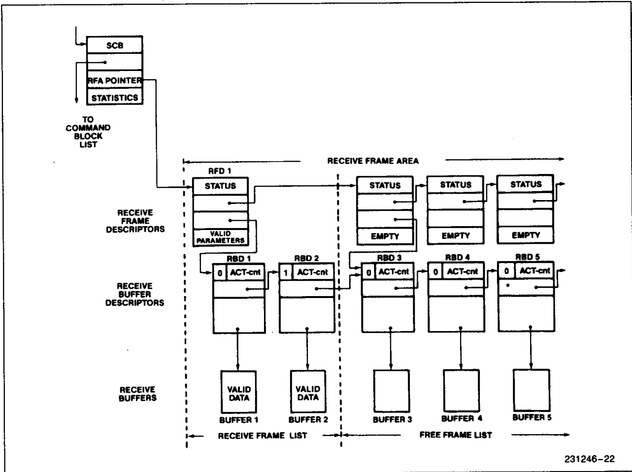
Figure 21. The Receive Frame Area
