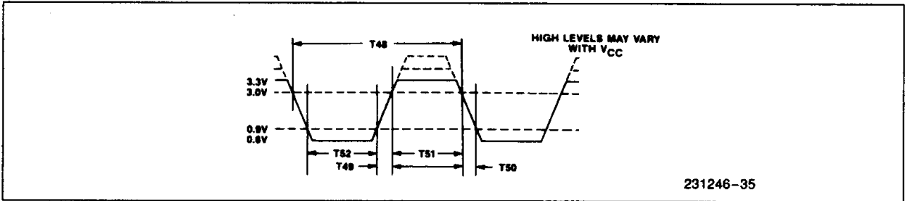
Figure 34. \overline{\text{Tx}}\text{C} Input Voltage Levels for Timing Measurements
