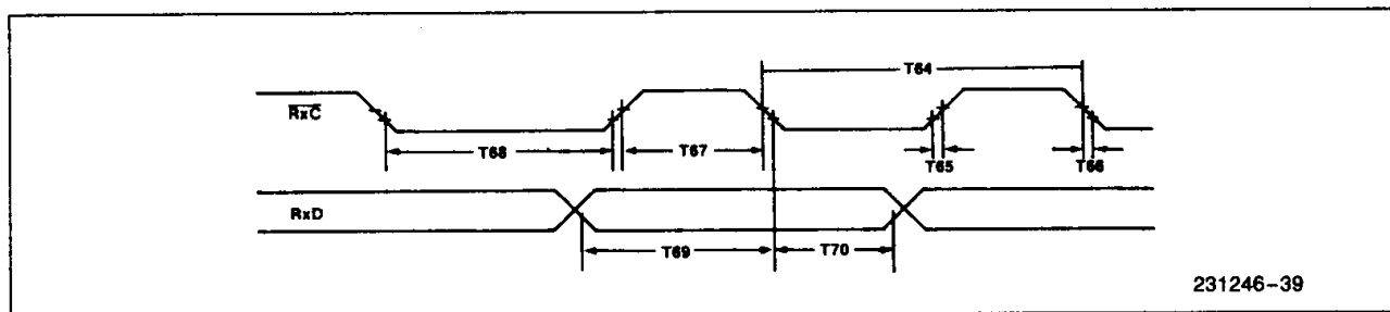
Figure 37. RxD Timing Relative to \overline{RxC}
