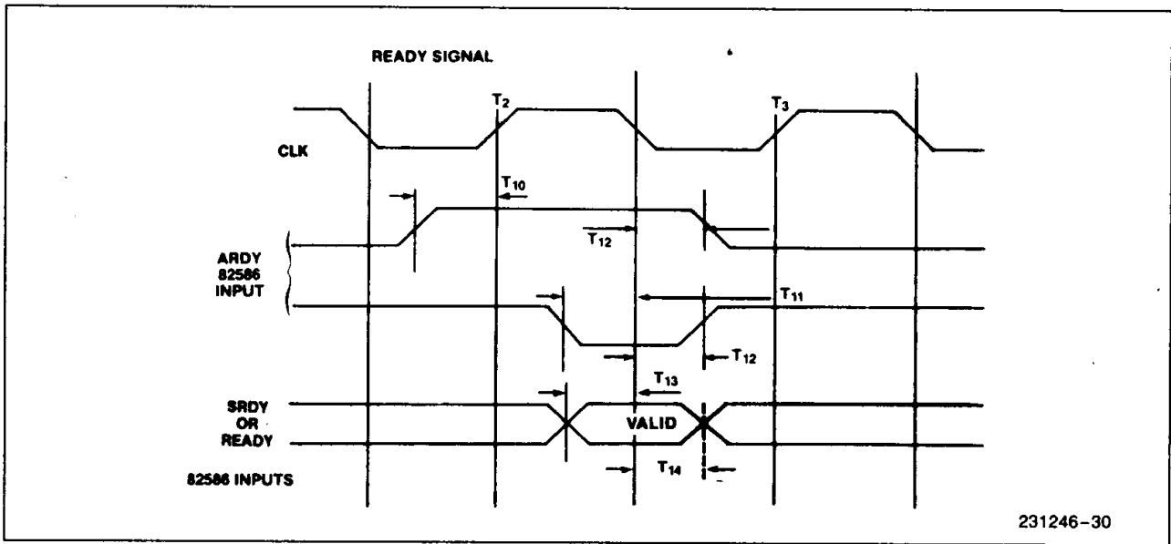
Figure 29. ARDY and SRDY Timings Relative to CLK
