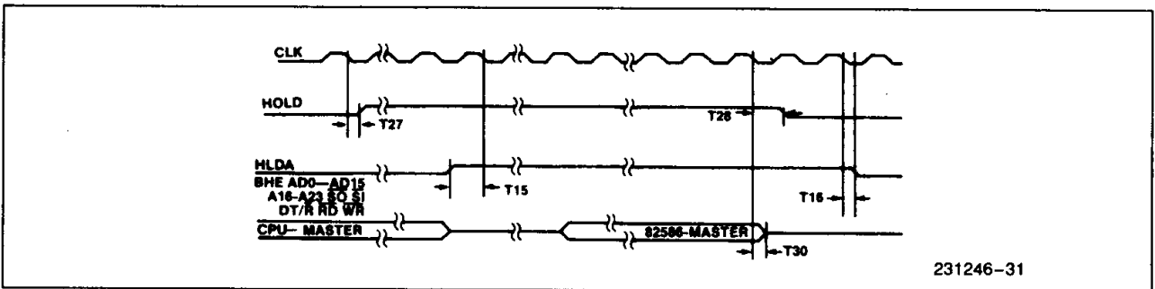
Figure 30. HOLD/HLDA Timing Relative to CLK
