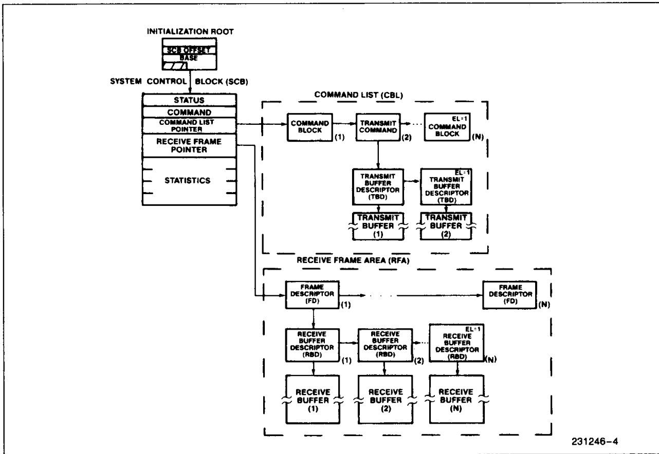
Figure 4. 82586 Shared Memory Structure
