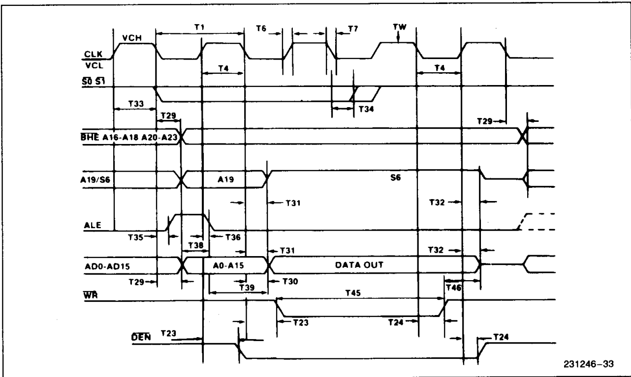
Figure 32. Write Cycle Timing
