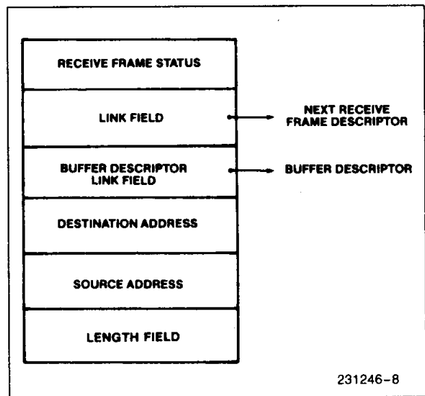
Figure 9. Receive Frame Descriptor
