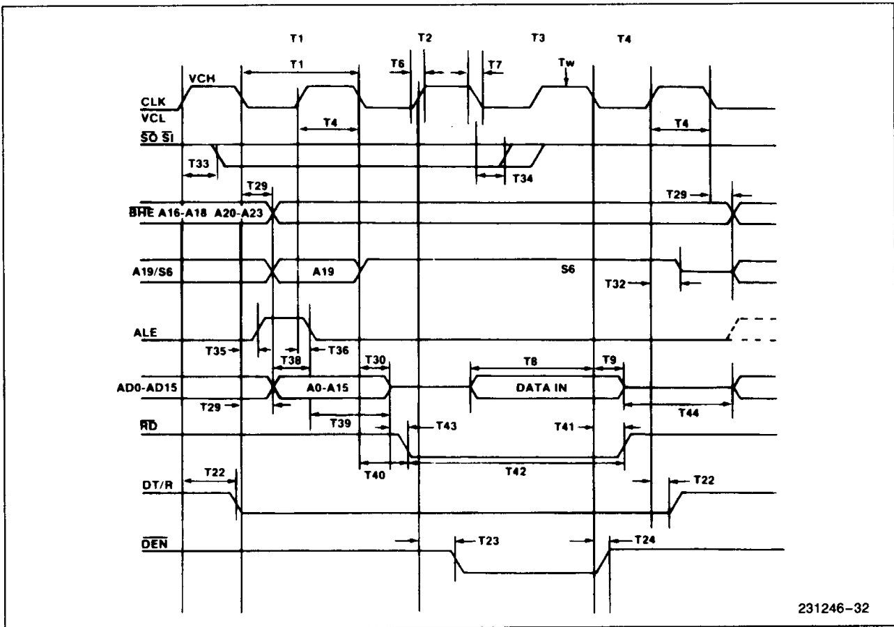
Figure 31. Read Cycle Timing
