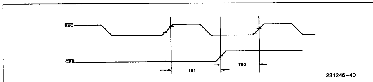
Figure 38. CRS Timing Relative to \overline{RxC}
