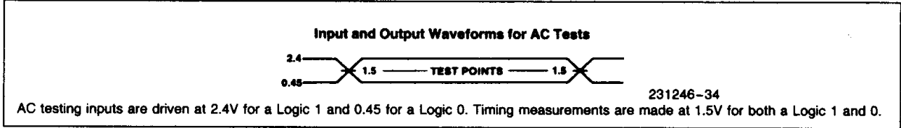
Figure 33. TTL Input/Output Voltage Levels for Timing Measurements
