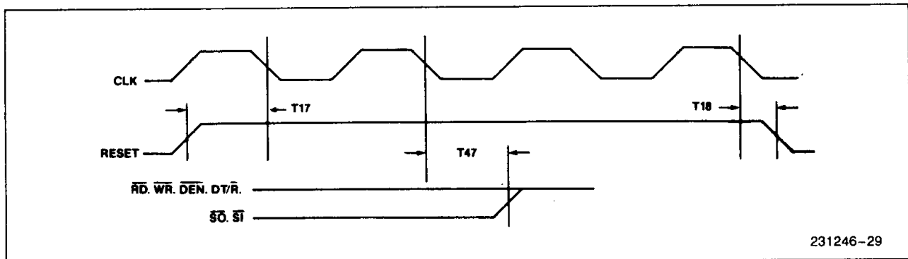
Figure 28. RESET Timing
