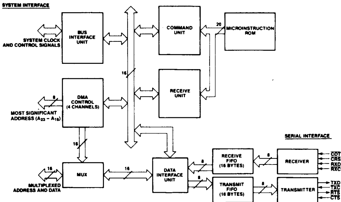
Figure 1. 82586 Functional Block Diagram
