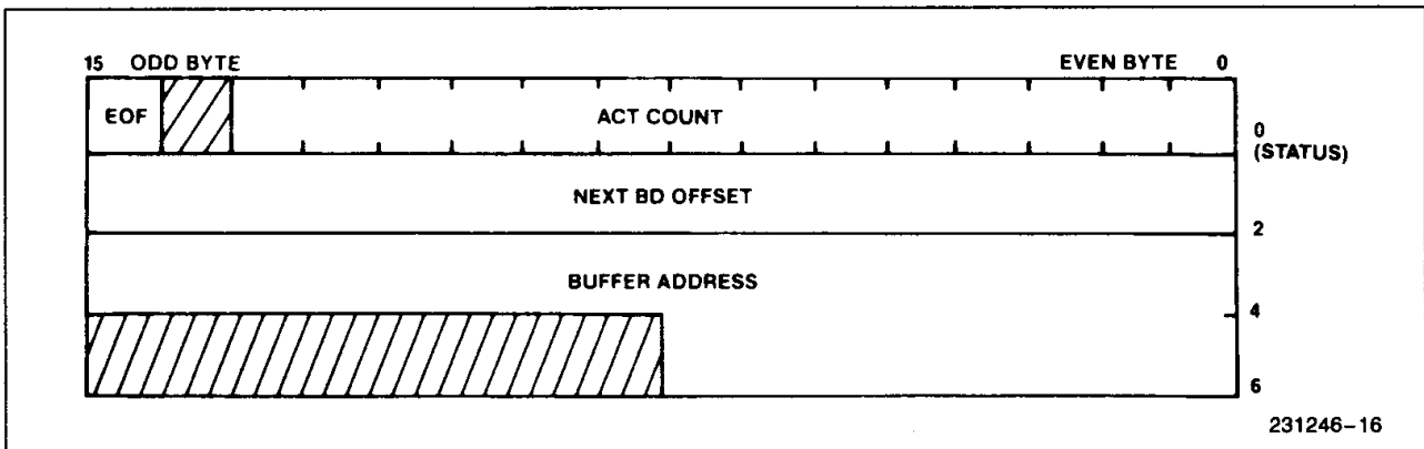
Figure 16. The Transmit Buffer Description
