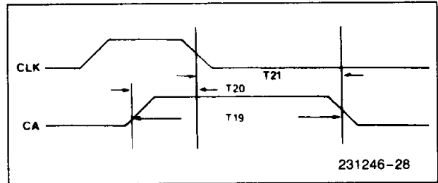
Figure 27. CA Input Timing
