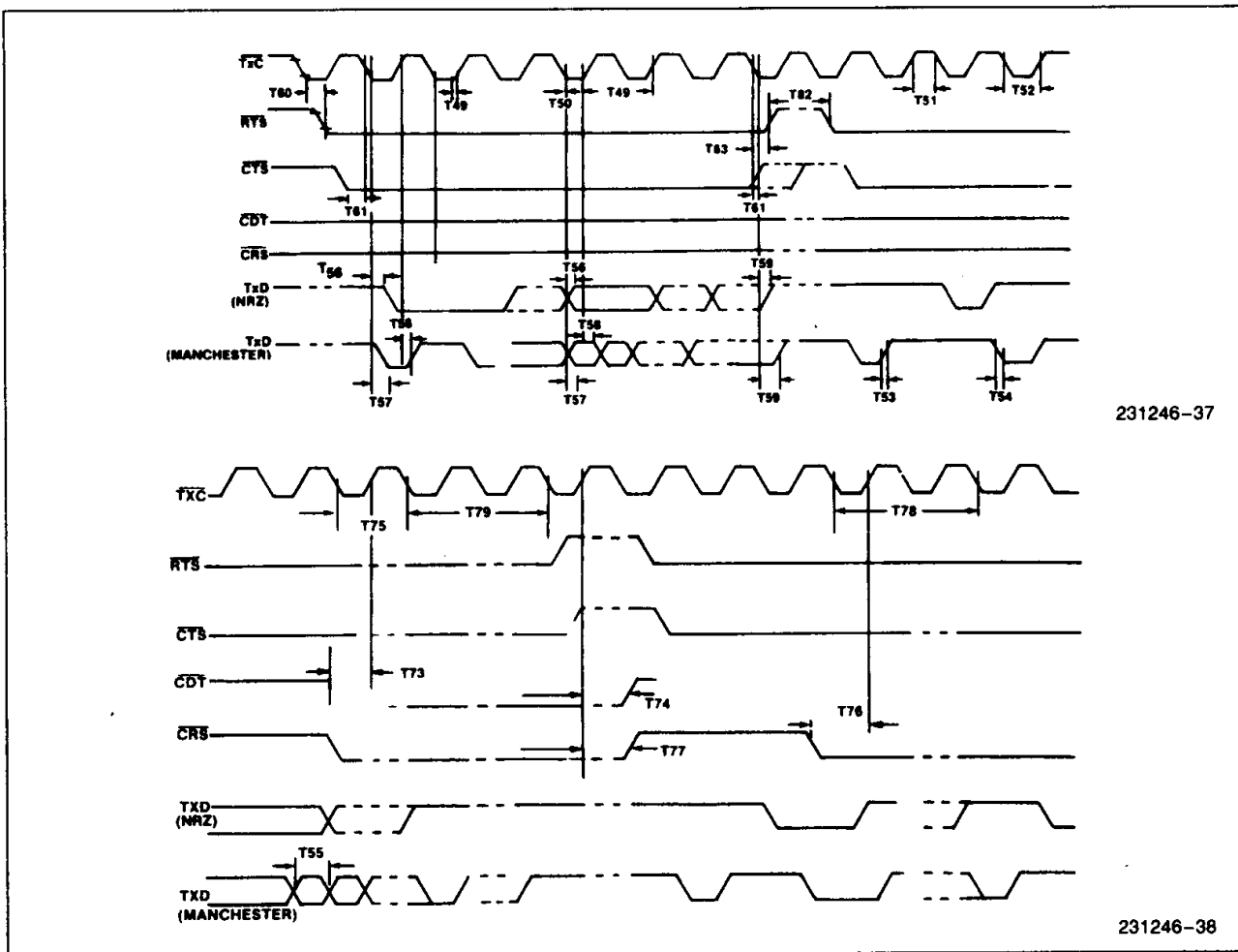
Figure 36. Transmit and Control and Data Timing
