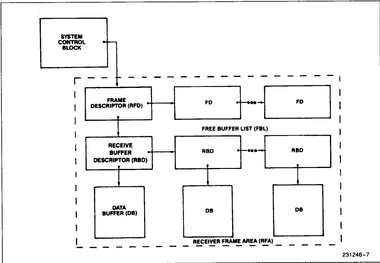
Figure 8. Receive Frame Area Diagram
