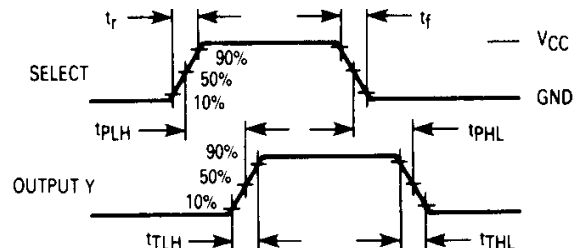
Figure 2. Switching Waveforms
