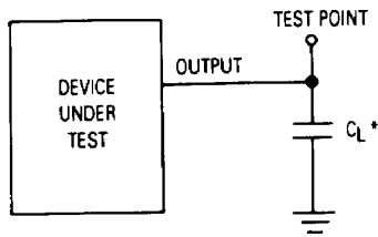
Figure 3. Test Circuit
