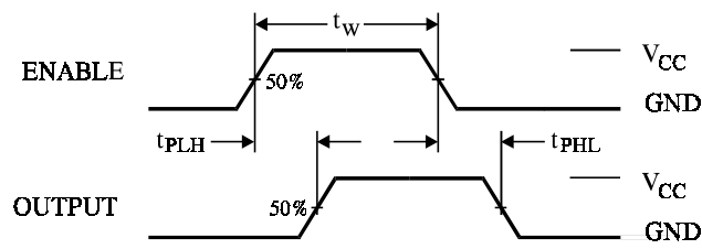
Figure 3. Switching Waveforms
