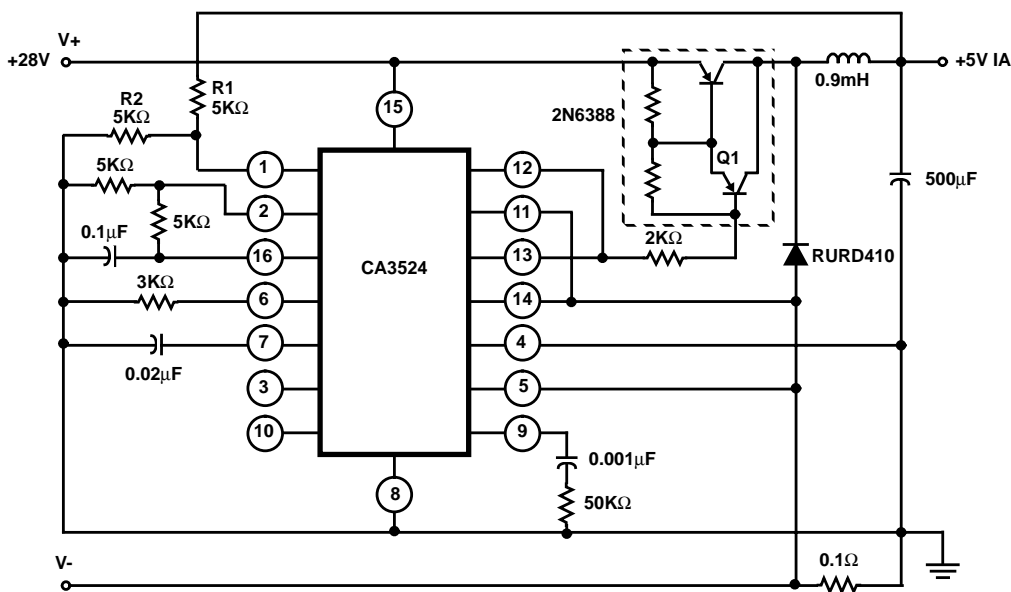
FIGURE 19. SINGLE-ENDED LC SWITCHING REGULATOR CIRCUIT
