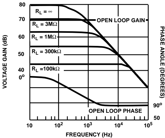
FIGURE 6. OPEN-LOOP ERROR AMPLIFIER RESPONSE CHARACTERISTICS.
