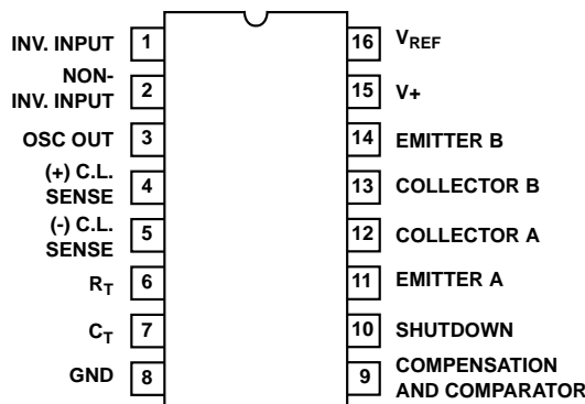
CA1524, CA2524, CA3524 (PDIP, CERDIP) TOP VIEW
