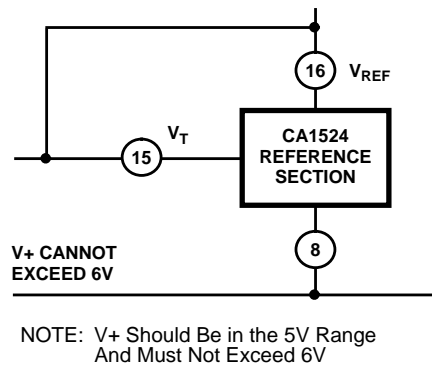
FIGURE 12. CIRCUIT TO ALLOW EXTERNAL BYPASS OF THE REFERENCE REGULATION
