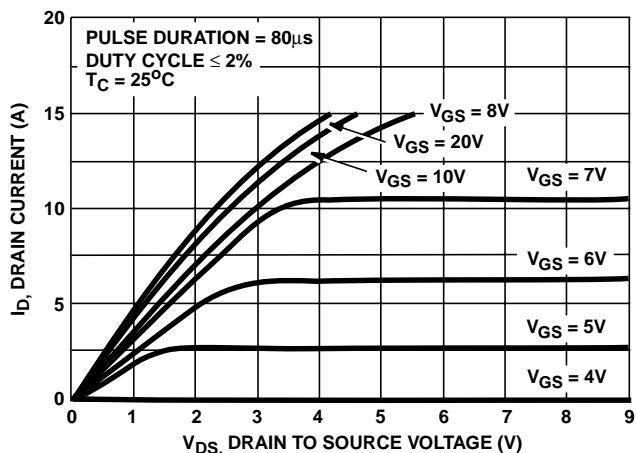
FIGURE 4. SATURATION CHARACTERISTICS
