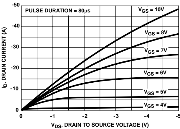
FIGURE 6. SATURATION CHARACTERISTICS
