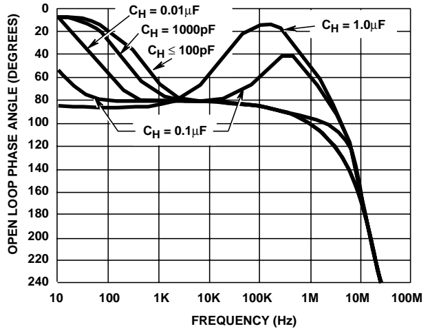
FIGURE 15. OPEN LOOP PHASE RESPONSE
