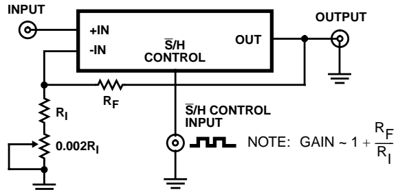
FIGURE 7. NON-INVERTING CONFIGURATION
