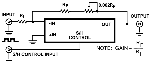
FIGURE 6. INVERTING CONFIGURATION
