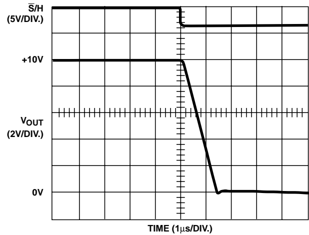
FIGURE 17. ACQUISITION TIME ( C_H = 1000\text{pF} )
