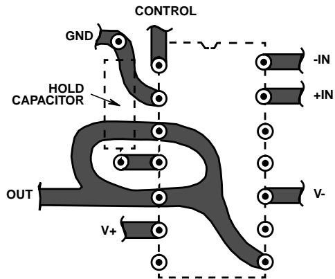
FIGURE 9. GUARD RING LAYOUT (BOTTOM VIEW)
