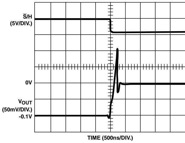
FIGURE 20. ACQUISITION TIME ( C_H = 1000\text{pF} )
