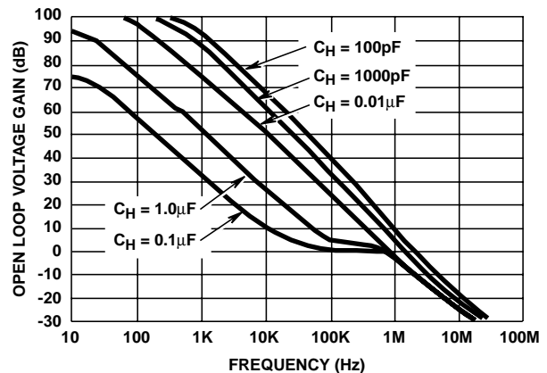
FIGURE 13. OPEN LOOP FREQUENCY RESPONSE
