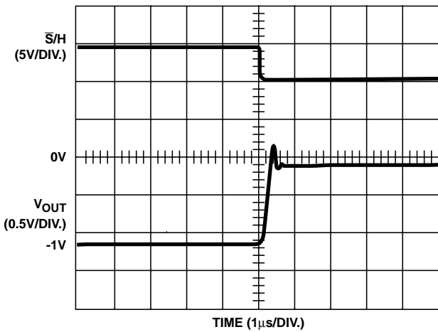
FIGURE 18. ACQUISITION TIME ( C_H = 1000\text{pF} )
