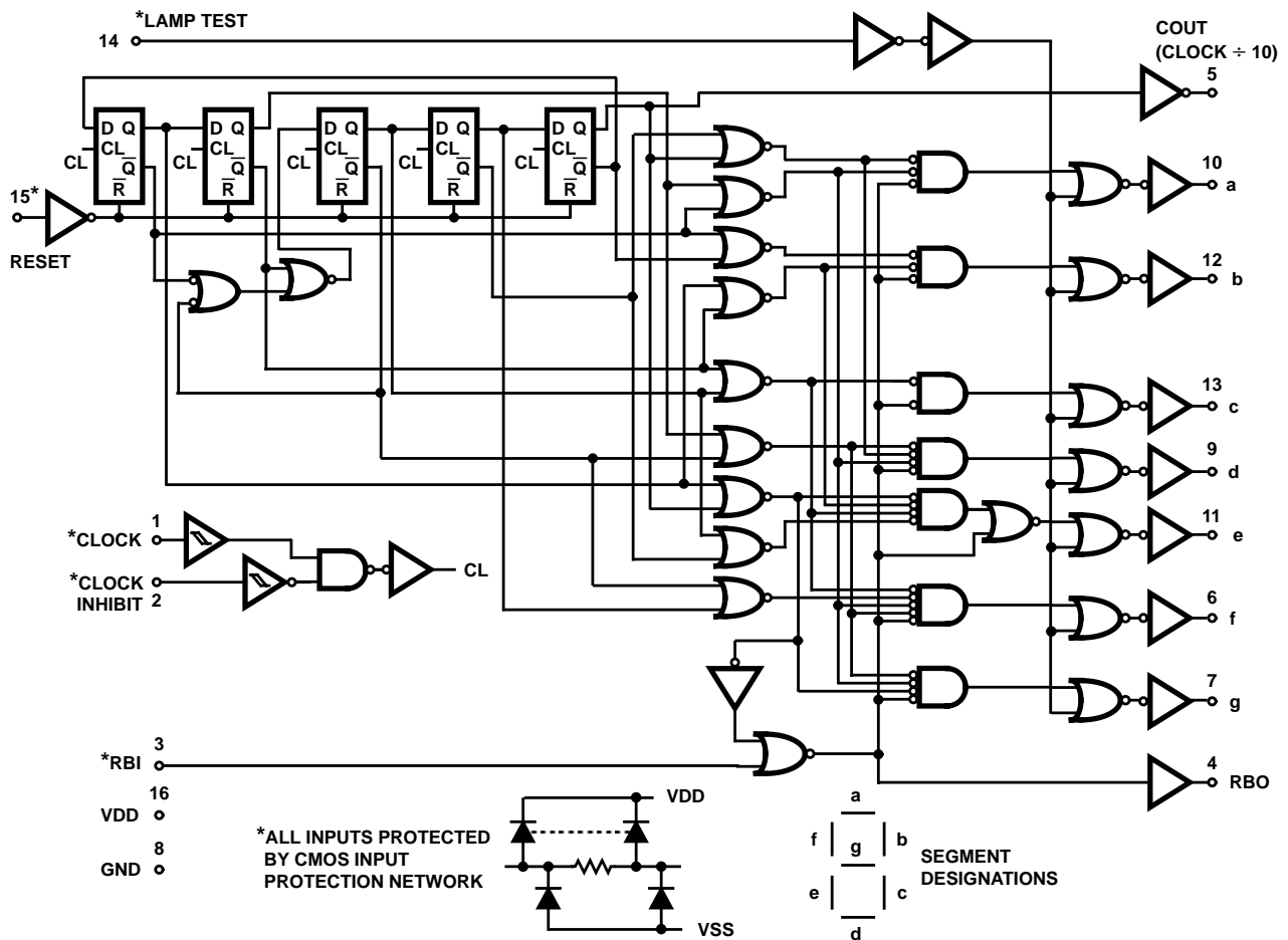
FIGURE 1. CD4033BMS
