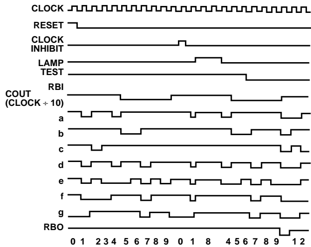
FIGURE 2. CD4033BMS TIMING DIAGRAM
