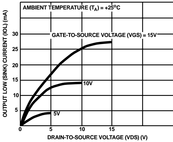
FIGURE 4. TYPICAL N-CHANNEL OUTPUT LOW (SINK) CURRENT CHARACTERISTICS
