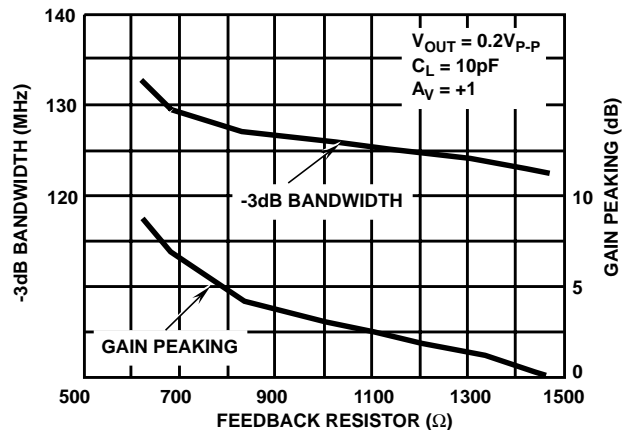
FIGURE 4. BANDWIDTH AND GAIN PEAKING vs FEEDBACK RESISTANCE
