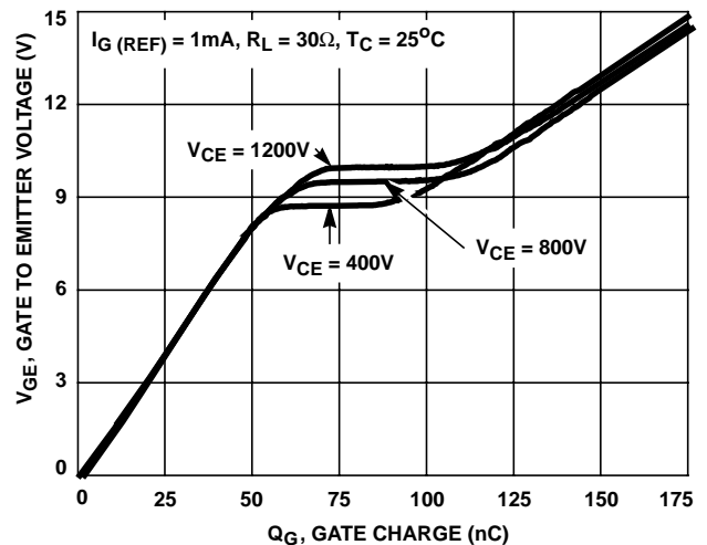
FIGURE 14. GATE CHARGE WAVEFORMS
