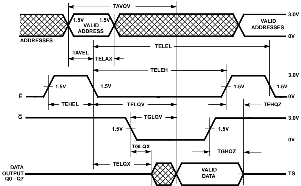
FIGURE 1. READ CYCLE
