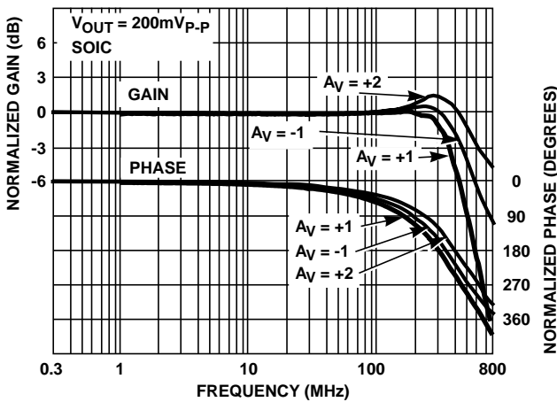
FIGURE 12. FREQUENCY RESPONSE
