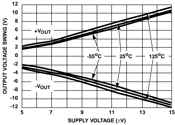
FIGURE 14. OUTPUT VOLTAGE SWING vs SUPPLY VOLTAGE
