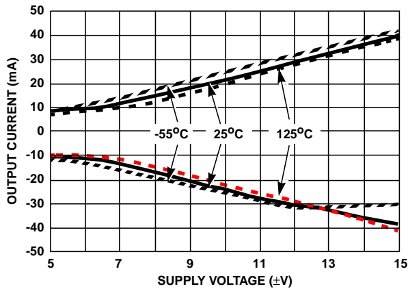
FIGURE 16. OUTPUT CURRENT vs SUPPLY VOLTAGE
