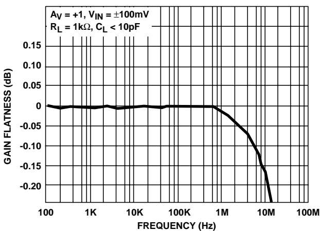
FIGURE 24. GAIN FLATNESS
