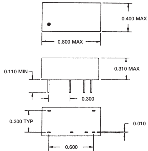
Dual-In-Line-Package
