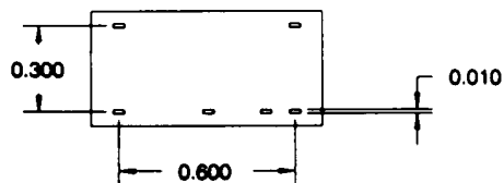
DUAL-IN-LINE PACKAGE
